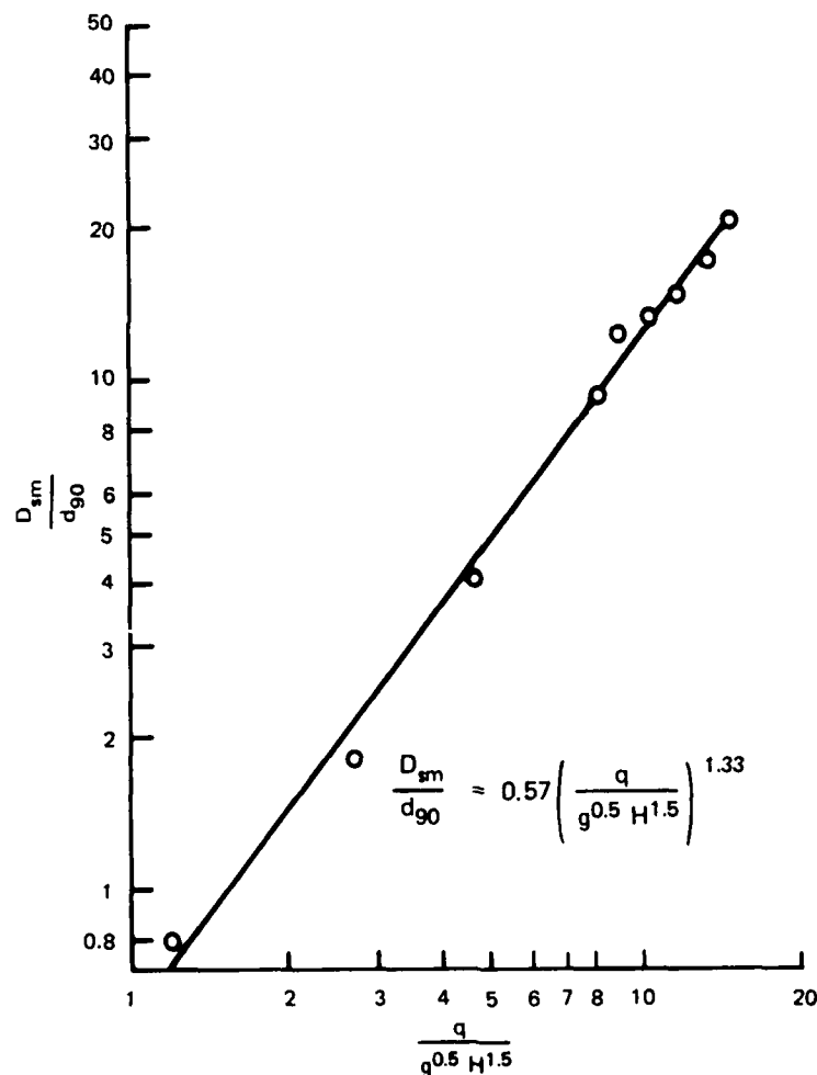
Figure 15. Relation between scour depth and unit discharge for Mill Creek channel
