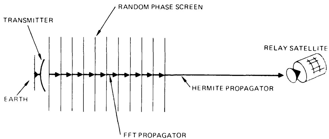
Figure 2. Turbulence modeling.
