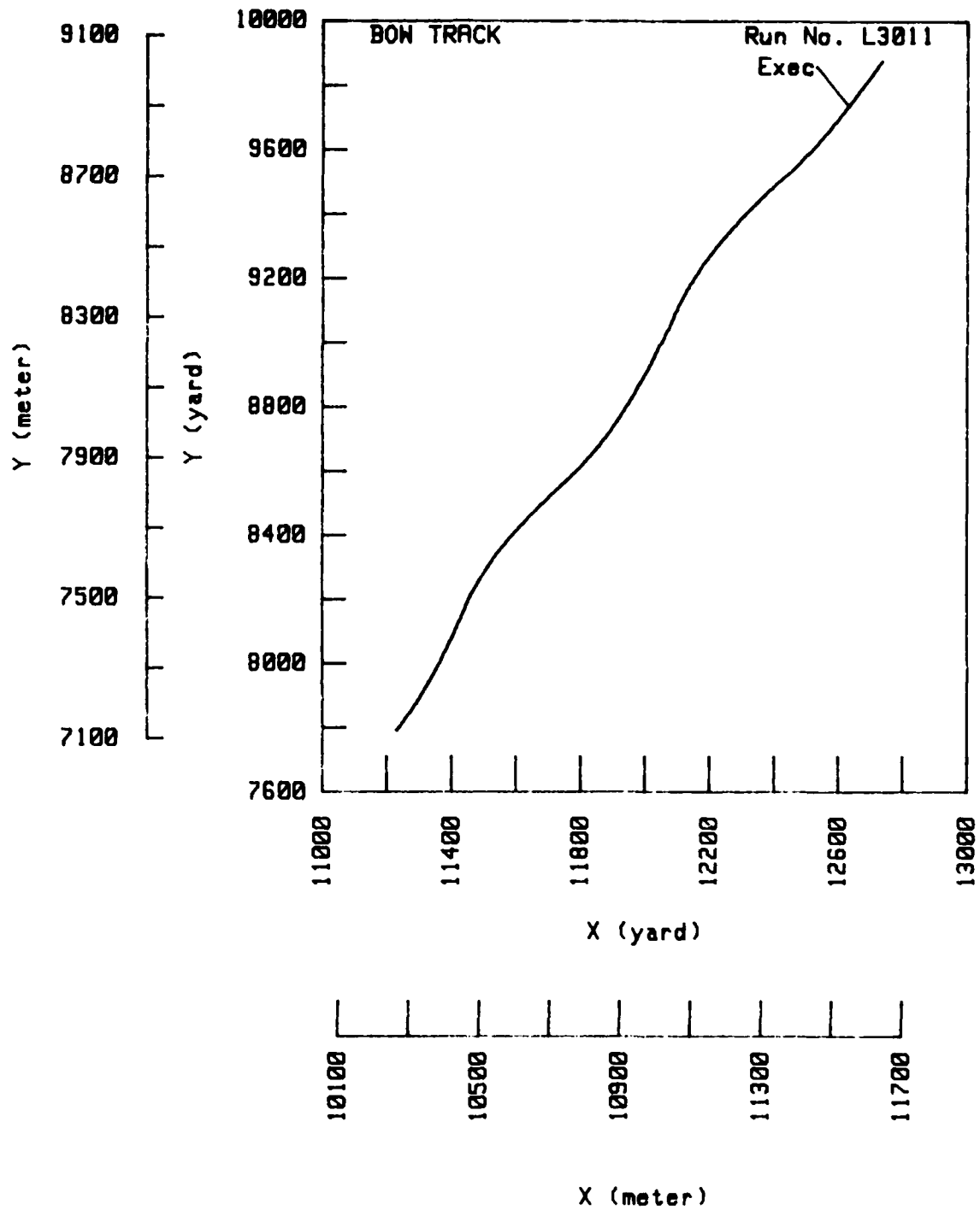
Figure 97 - Position Plot for Full Ahead, 10/10 Degrees Overshoot Maneuver (Run L3011)
