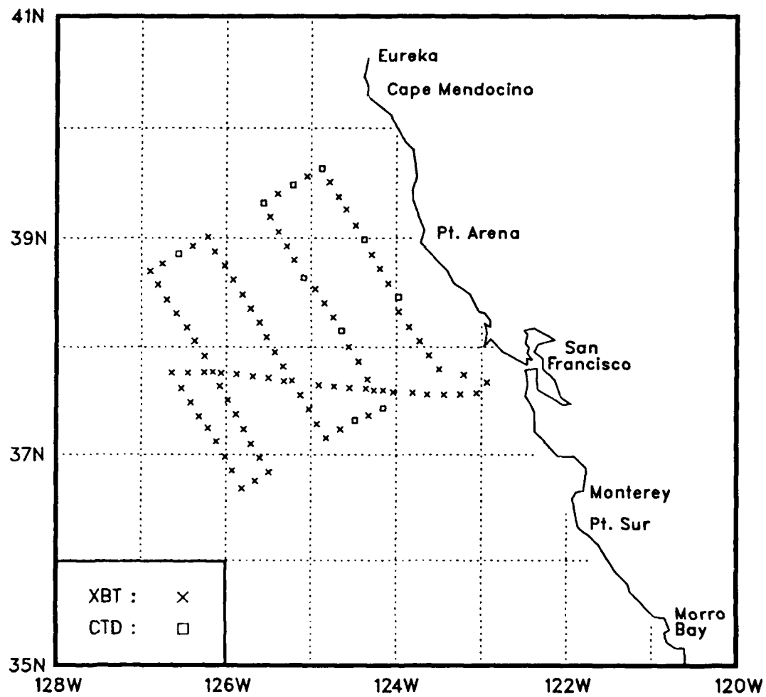
Figure 3: XBT and CTD locations for OPTOMA19.
