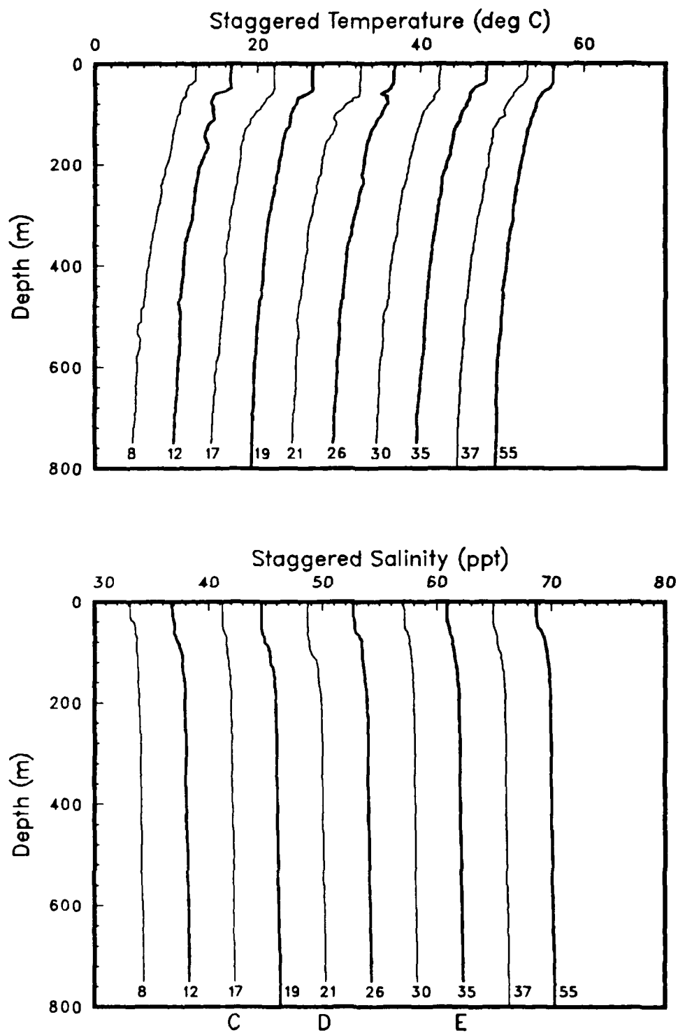
Figure 6(a): CTD temperature profiles, staggered by multiples of 5C, and salinity profiles staggered by multiples of 4 ppt (OPTOMA19).
