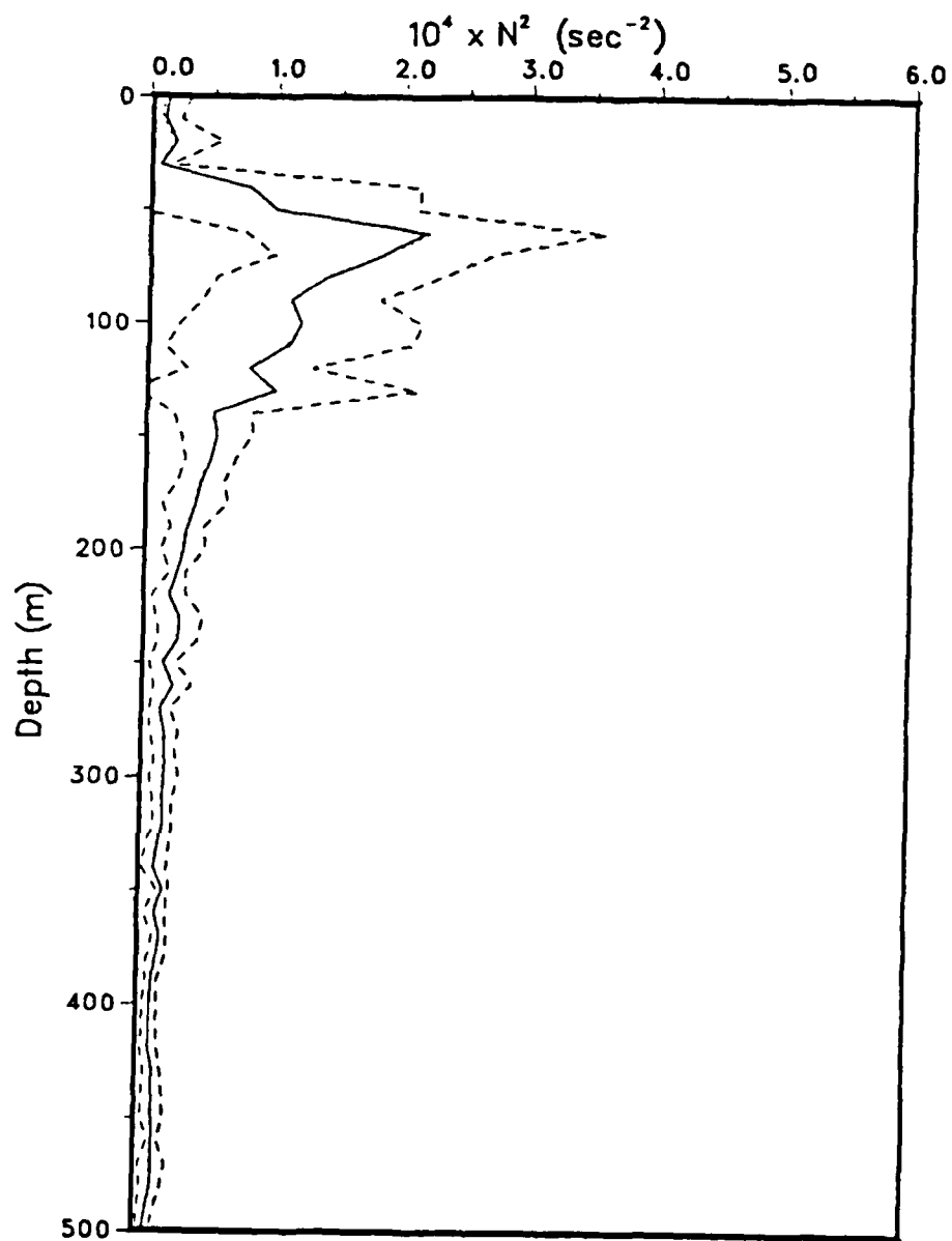
Figure 12: Profile of N^2(z) (—), with + and - the standard deviation (---), and the profile of N^2 from \overline{T(z)} and \overline{S(z)} (...) (OPTOMA19).
