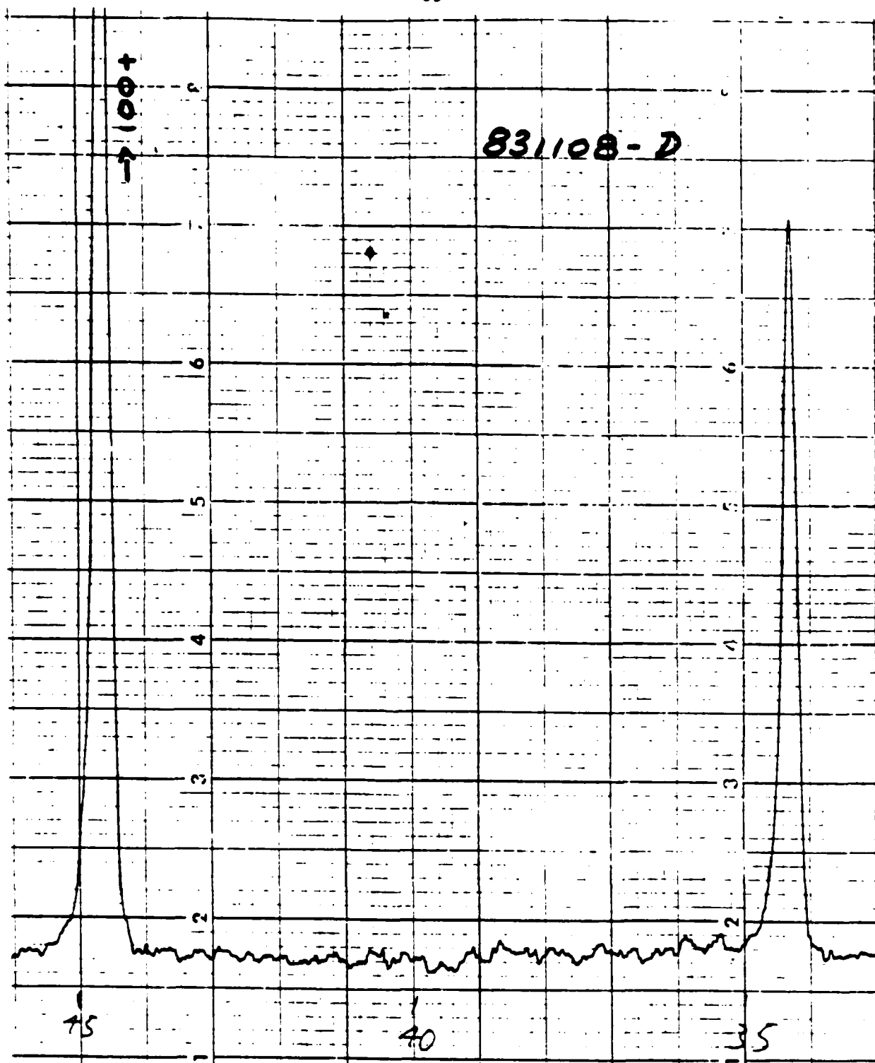
X-Ray Powder Diffraction Pattern for TiB 2 (Experiment XXI)
