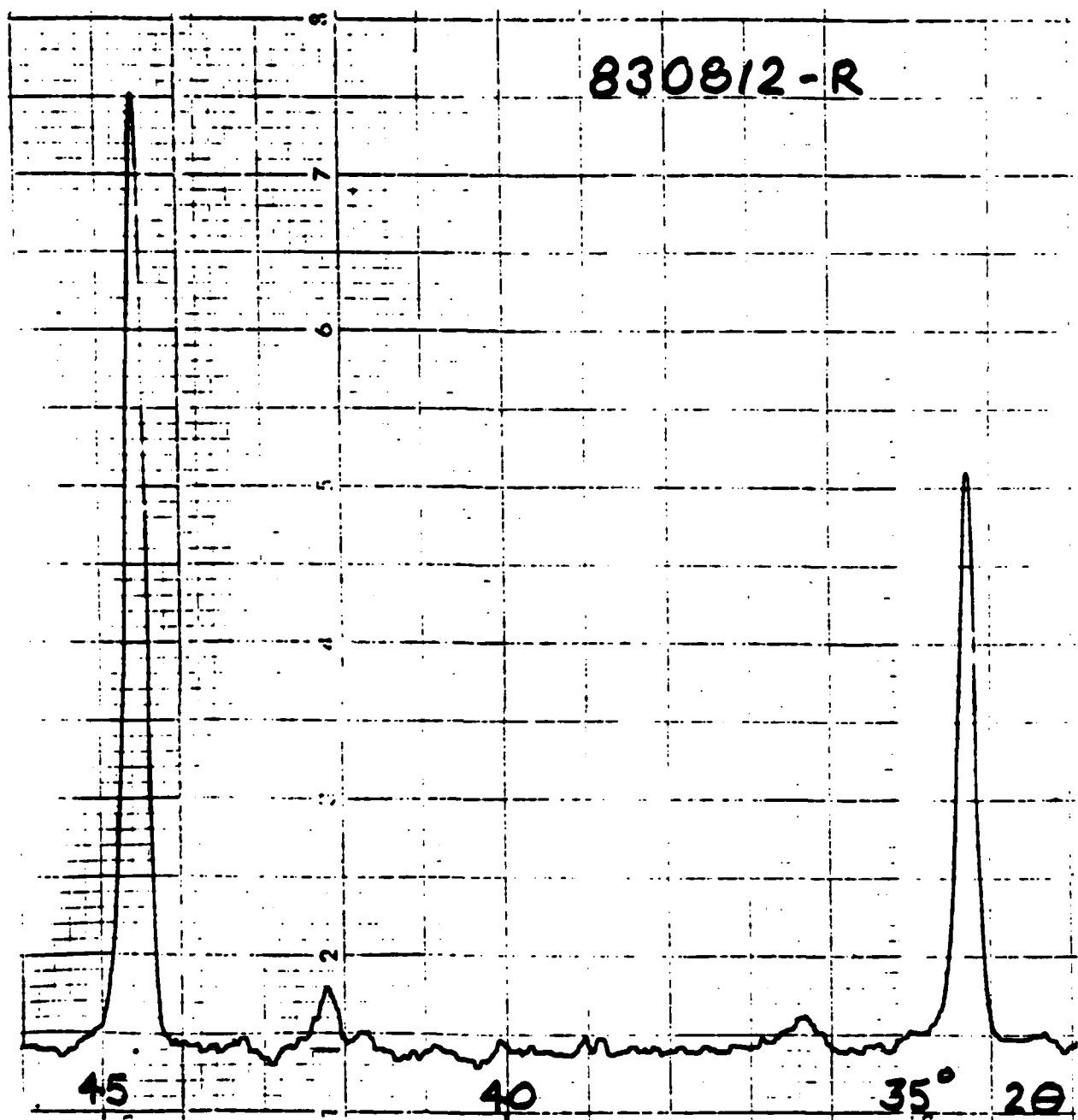
X-Ray Powder Diffraction Pattern for \text{TiB}_2 (Experiment III)
