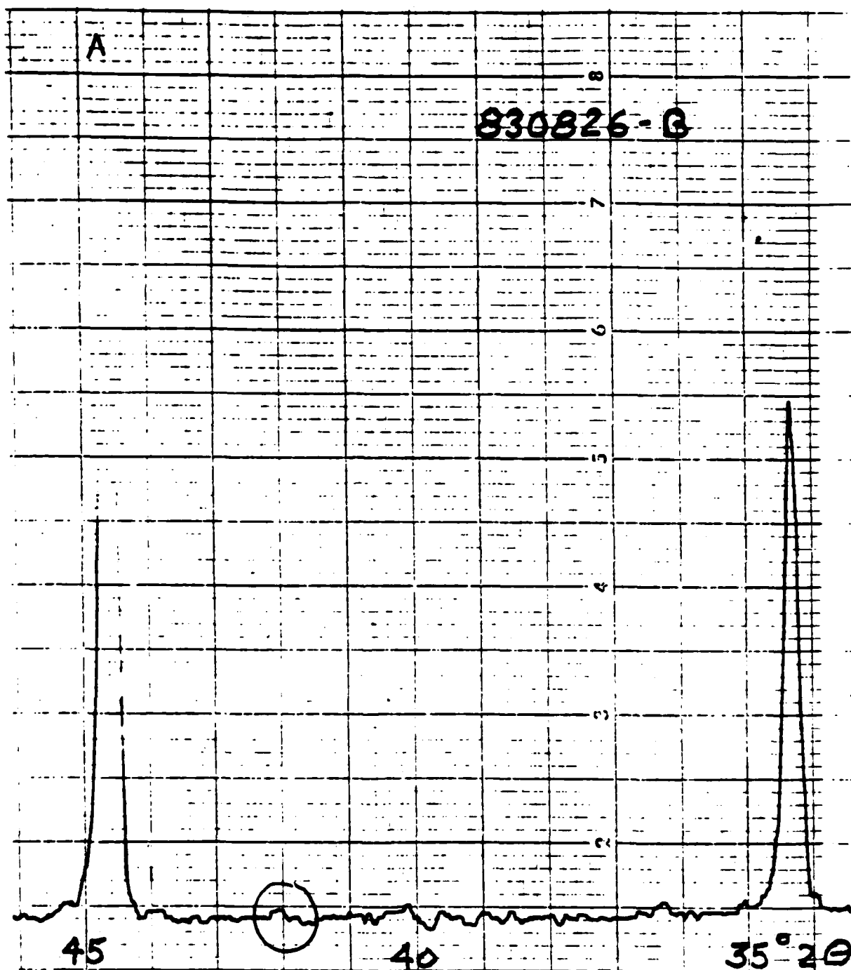
X-Ray Powder Diffraction Pattern for TiB 2 (Experiment VII)
