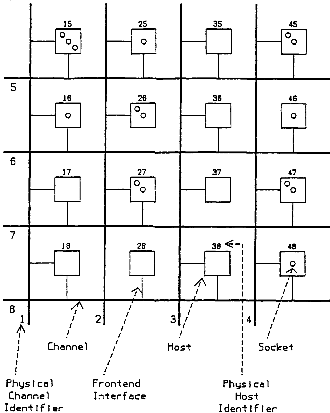
Figure 4. An example of a netcomputer
