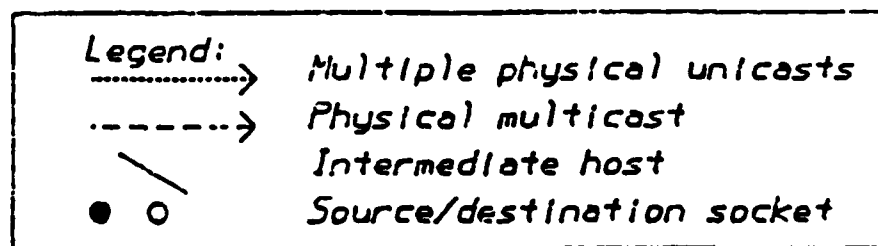
Figure 7. Example of channel multicast from host 46 to group hosts on channels 4,5 and 7
