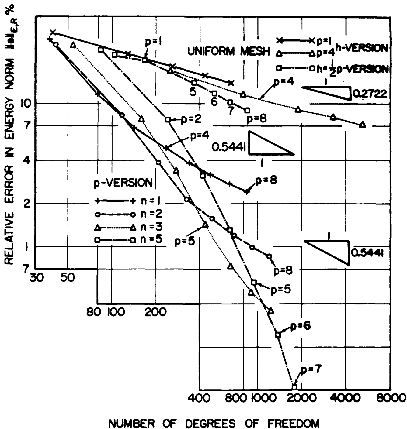
Fig. 6.7. The error in the energy norm in dependence on N for various meshes.
