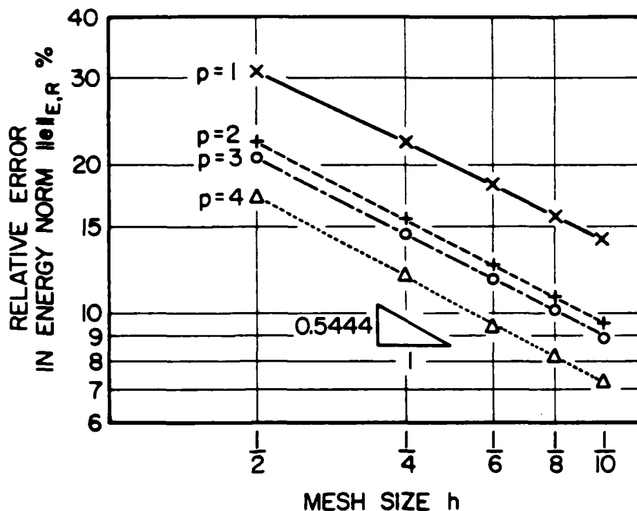
Fig. 6.3. The relative error in the energy norm in dependence on h .
