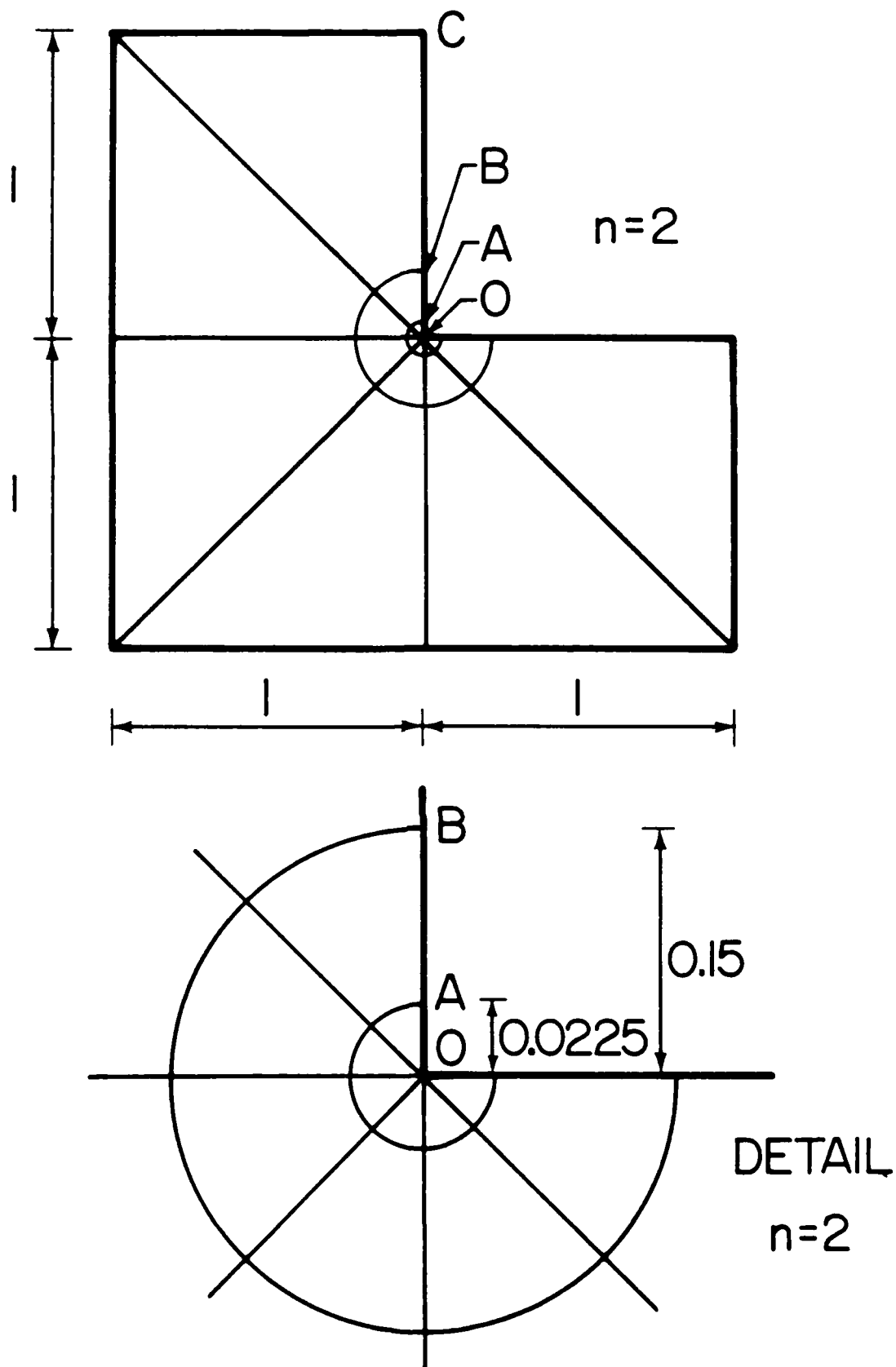
Fig. 6.6. The strongly refined mesh with n = 2 layers.
