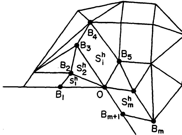
Fig. 5.2. Scheme of the mesh in the neighborhood of the singularity.
