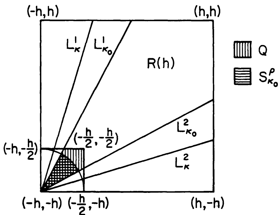
Fig. 5.1. Scheme of R(h) , Q , S_{\kappa_0}^p .
