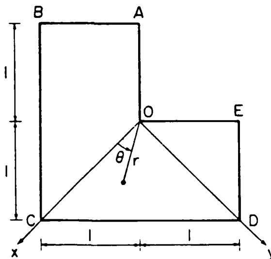
Fig. 6.1. L-shaped plane elastic body.
