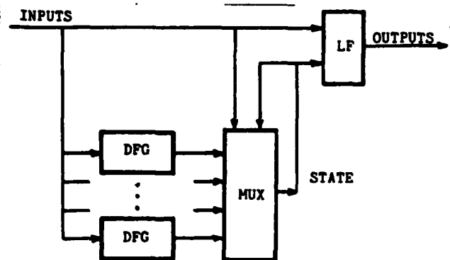
FIGURE 1. THE SAM ARCHITECTURE
