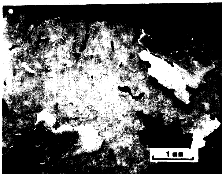
Figure 58: Photograph showing some of the large Al 2 O 3 scale flakes spalled off from the undoped NiCrAl specimen oxidized for 24 hours at 1100°C.
