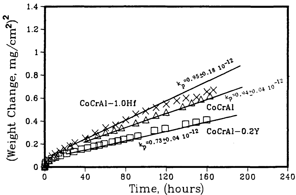
Figure 21: (Continued), weight change squared vs time plot for isothermally oxidized specimens at 1100°C, (c) CoCrAl alloys doped with yttrium or hafnium. Values of parabolic rate constant ( k_p ) are given in \text{gm}^2/\text{cm}^4\text{-sec} .
