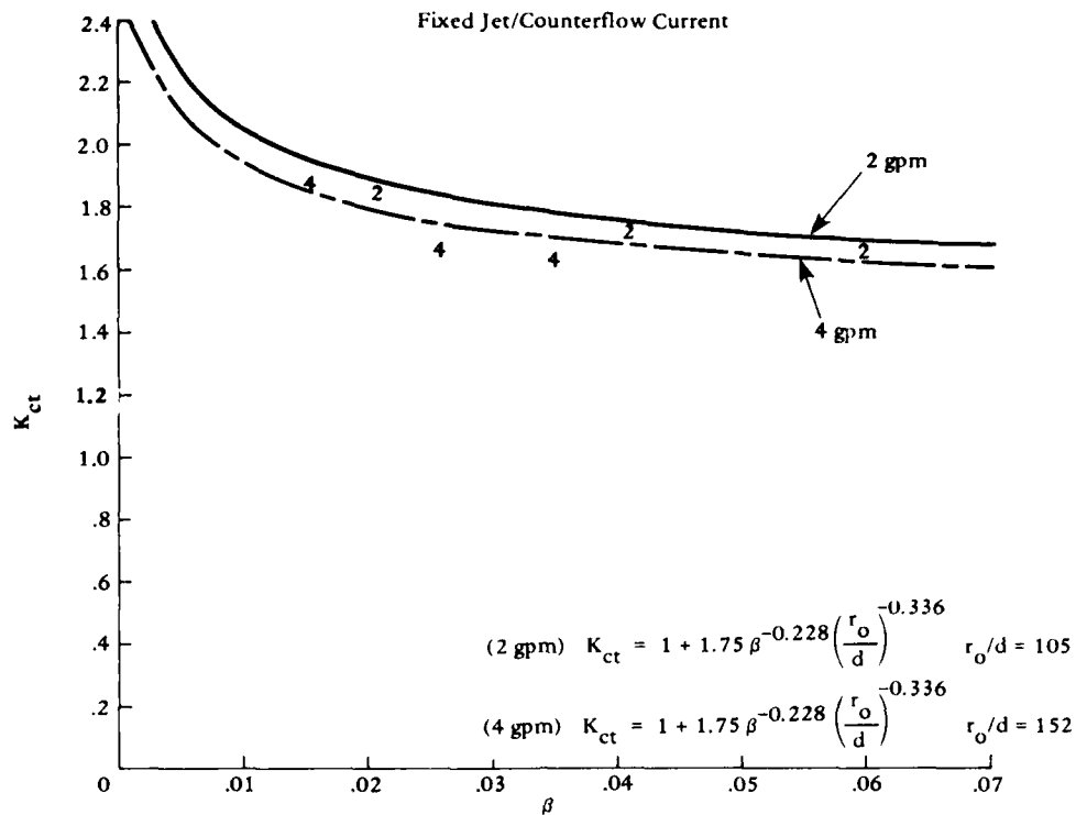
Figure 13. Equations and graph for predicting scour radius given a jet (discharge rate and diameter) and a mean current velocity.
