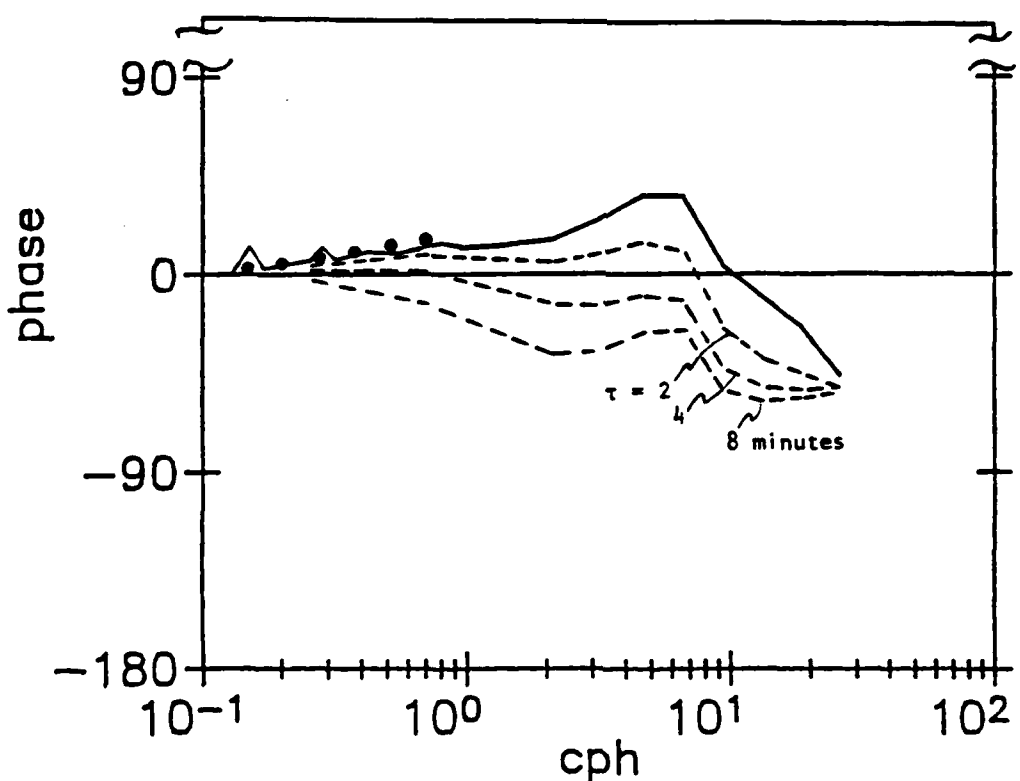
Fig. 5. Coherence and phase between conductivity and temperature measured at 257 m on the central mooring (solid line). Phase between conductivity and filtered temperature using \tau = 2, 4, and 8 minutes is plotted with a dashed line. Phase modeled by equation (3) with \tau = 4 minutes is shown by a dotted line.
