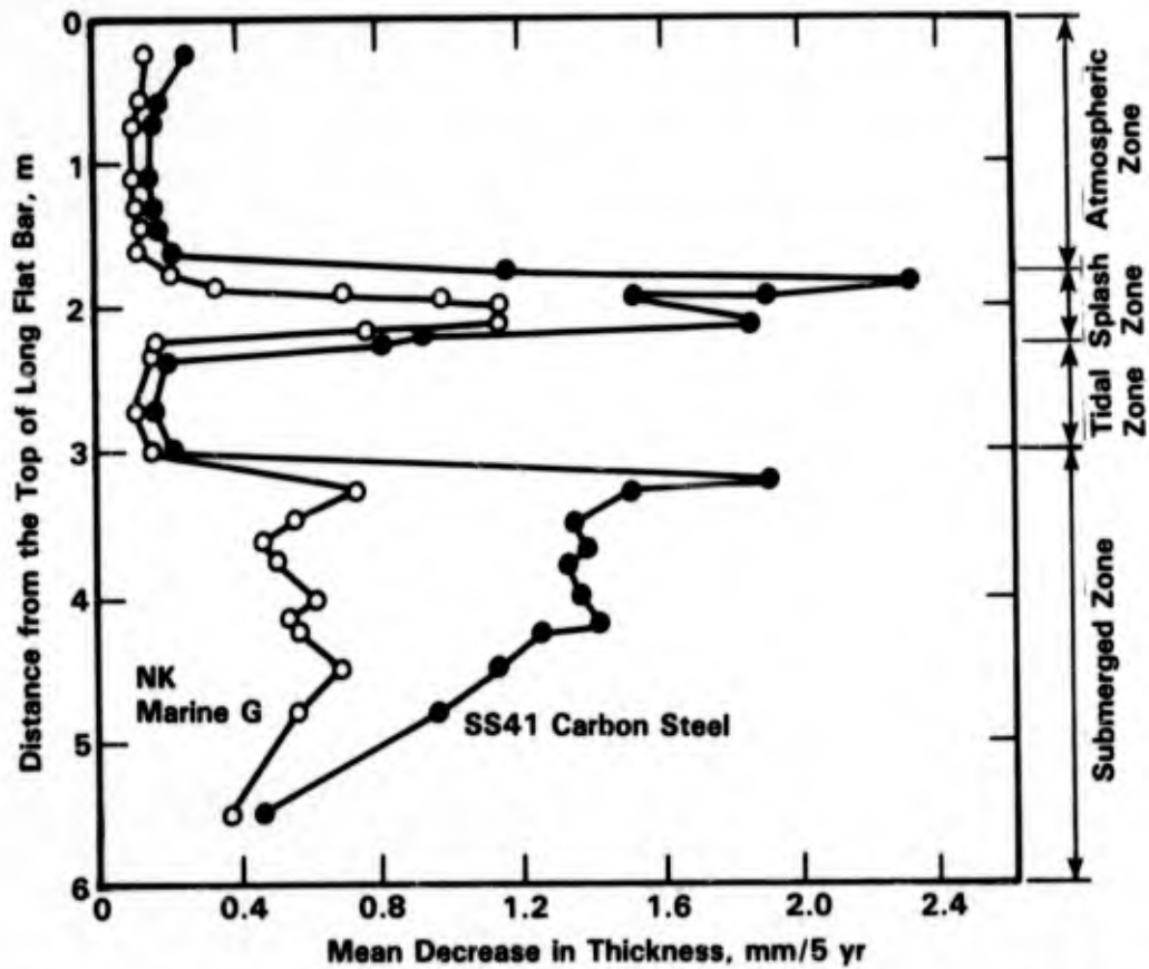
FIGURE 6-11. RESULT OF SEAWATER CORROSION TEST ON LONG FLAT BARS FOR 5 YEARS AT SHIMIZU SHIPYARD, JAPAN. THE COMPOSITION OF NK MARINE G IS GIVEN IN TABLE F-4, APPENDIX F(14)
