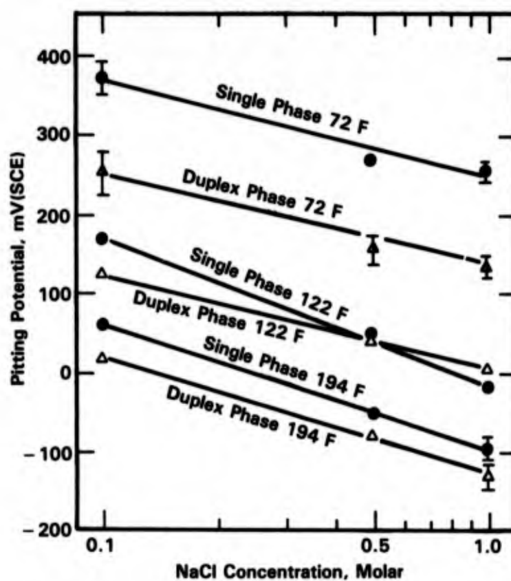
FIGURE 4-51. PITTING POTENTIALS OF SINGLE PHASE AND DUPLEX TYPE 304L AS A FUNCTION OF NaCl CONCENTRATION AT SEVERAL TEMPERATURES WITH A CONSTANT pH of 4 (119)
