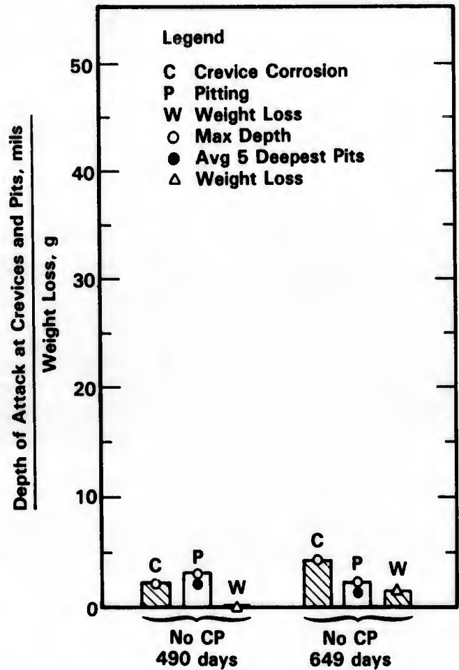
FIGURE 4-29. DEPTH OF ATTACK AND WEIGHT LOSS DATA ON STAINLESS STEEL No. 20Cb-3 IN SEAWATER AT KEY WEST, FL, WITHOUT CATHODIC PROTECTION (113)
