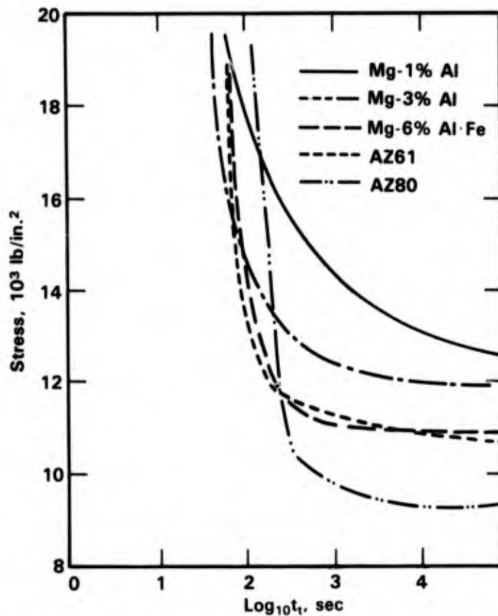
FIGURE 7-5. STRESS VERSUS TIME TO FAILURE ( t_f ) FOR Mg-Al ALLOYS IN AQUEOUS 40 g/l NaCl + 40 g/l \text{Na}_2\text{CrO}_4 (9)
