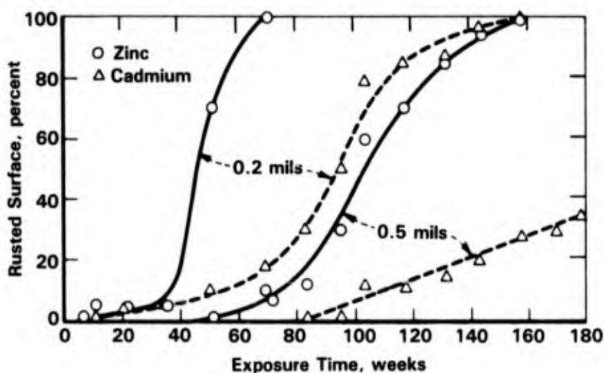
FIGURE 13-3. COMPARISON OF PROGRESSIVE DEVELOPMENT OF RUST ON ZINC- AND CADMIUM-PLATED STEEL PANELS AT 80-FOOT LOT, KURE BEACH, NC (8) Coating thicknesses 0.2 and 0.5 mils.
