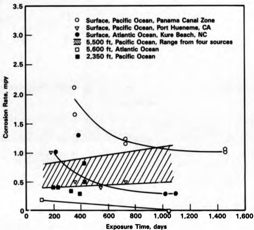
FIGURE 5-15. CORROSION OF NICKEL-COPPER ALLOY 400 IN SEAWATER (19)
