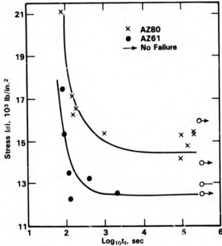
FIGURE 7-4. STRESS ( \sigma ) VERSUS TIME TO FAILURE ( t_f ) FOR THE TWO-PHASE ALLOYS AZ80 AND AZ61 IN AQUEOUS 40 g/l NaCl + 40 g/l \text{Na}_2\text{CrO}_4 (8)
