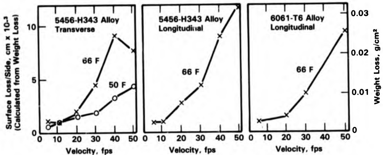
FIGURE 2-30. WEIGHT LOSS AND SURFACE RECESSION (CALCULATED FROM WEIGHT LOSS) AS A FUNCTION OF WATER VELOCITY FOR TWO ALUMINUM ALLOYS AFTER 30 DAYS IN SEAWATER (85)
