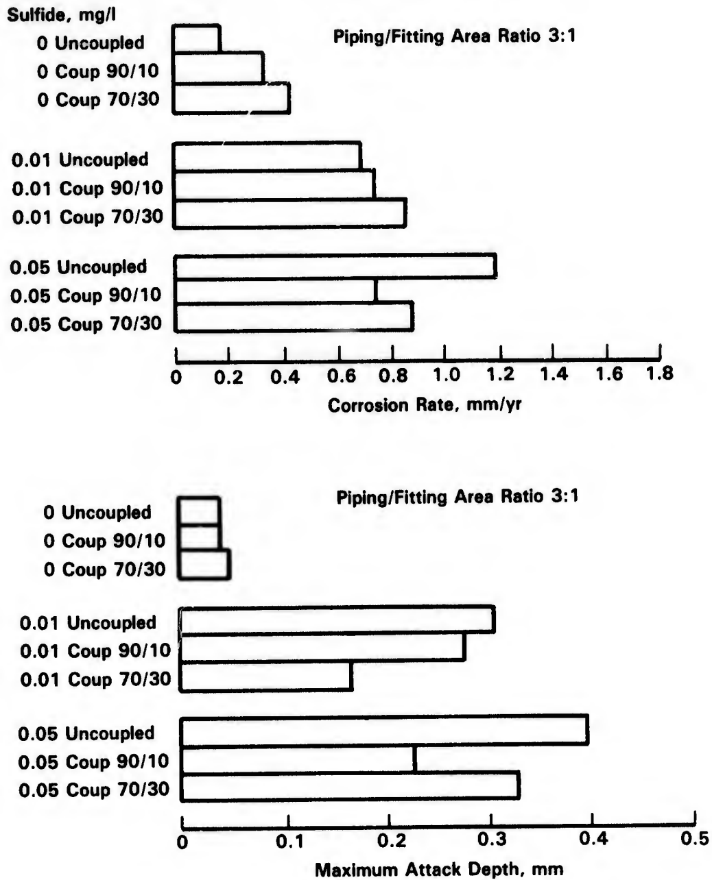
FIGURE 8-40. CORROSION OF Ni-Al-BRONZE COUPLED TO PIPING MATERIALS IN SULFIDE CONTAINING SEAWATER AT 2.4 M/S (64)
