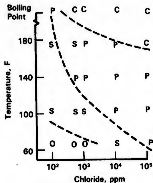
FIGURE 4-58. EFFECT OF CHLORIDE CONTENT AND TEMPERATURE ON TYPE OF CORROSION OF TYPE 304 IN SODIUM CHLORIDE SOLUTION: INITIAL pH 7 (136)
