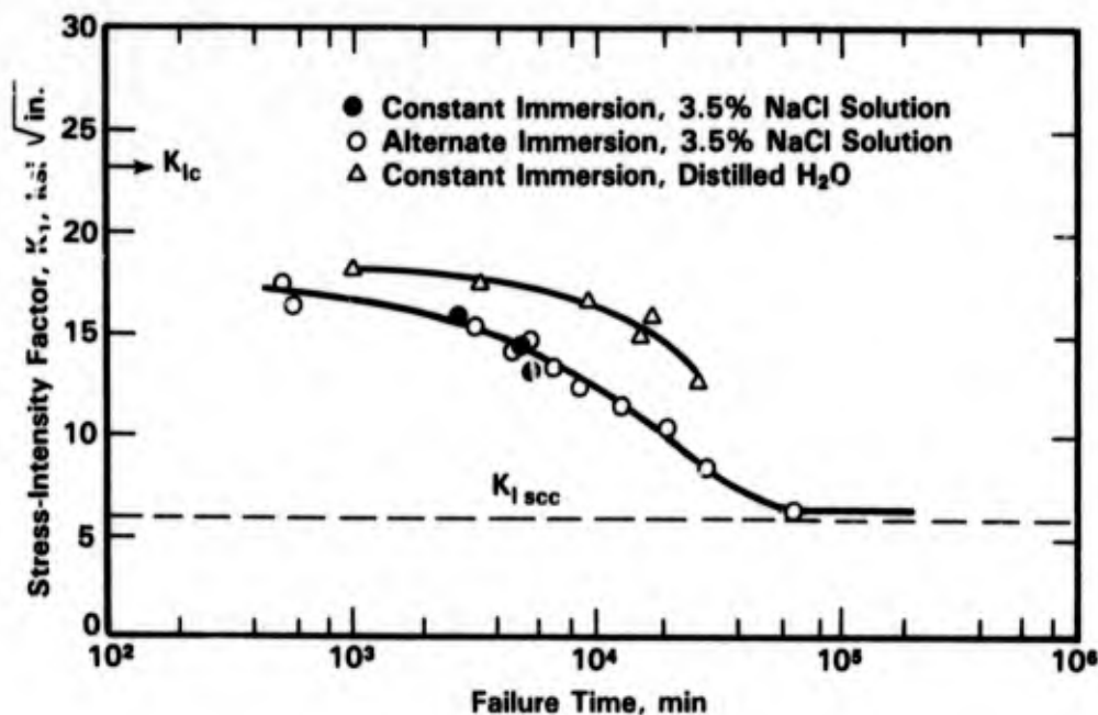
FIGURE 2-62. PRECRACKED-SPECIMEN STRESS-CORROSION DATA FOR SHORT TRANSVERSE 7075-T651 PLATE ILLUSTRATING THE TIME-TO-FAILURE METHOD OF OBTAINING K_{Isc} . USING THIS TECHNIQUE, A K_{Isc} OF ABOUT 6 KSI \sqrt{IN.} IS OBTAINED. (160)
