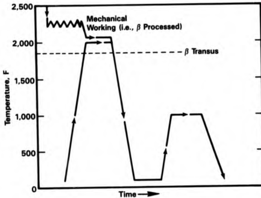
FIGURE 3-15. SCHEMATIC REPRESENTATION OF A \beta STA HEAT TREATMENT FOR Ti-6Al-4V. NOTE THAT THE \beta -PROCESSING PROCEDURE IS ALSO INDICATED. (75)
