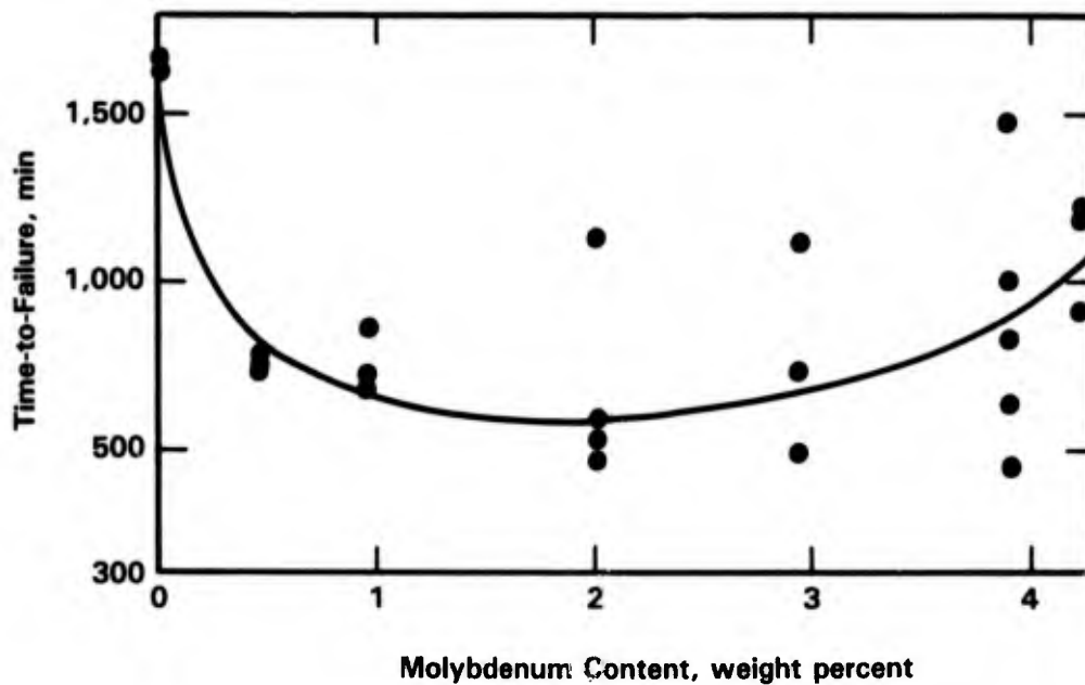
FIGURE 4-54. RESULTS OBTAINED ON 18Cr-14Ni-O to 4.2Mo STEELS STRESSED AT 75 PERCENT OF ROOM-TEMPERATURE YIELD STRENGTH IN BOILING MAGNESIUM CHLORIDE [140 C (284 F)] (131)
