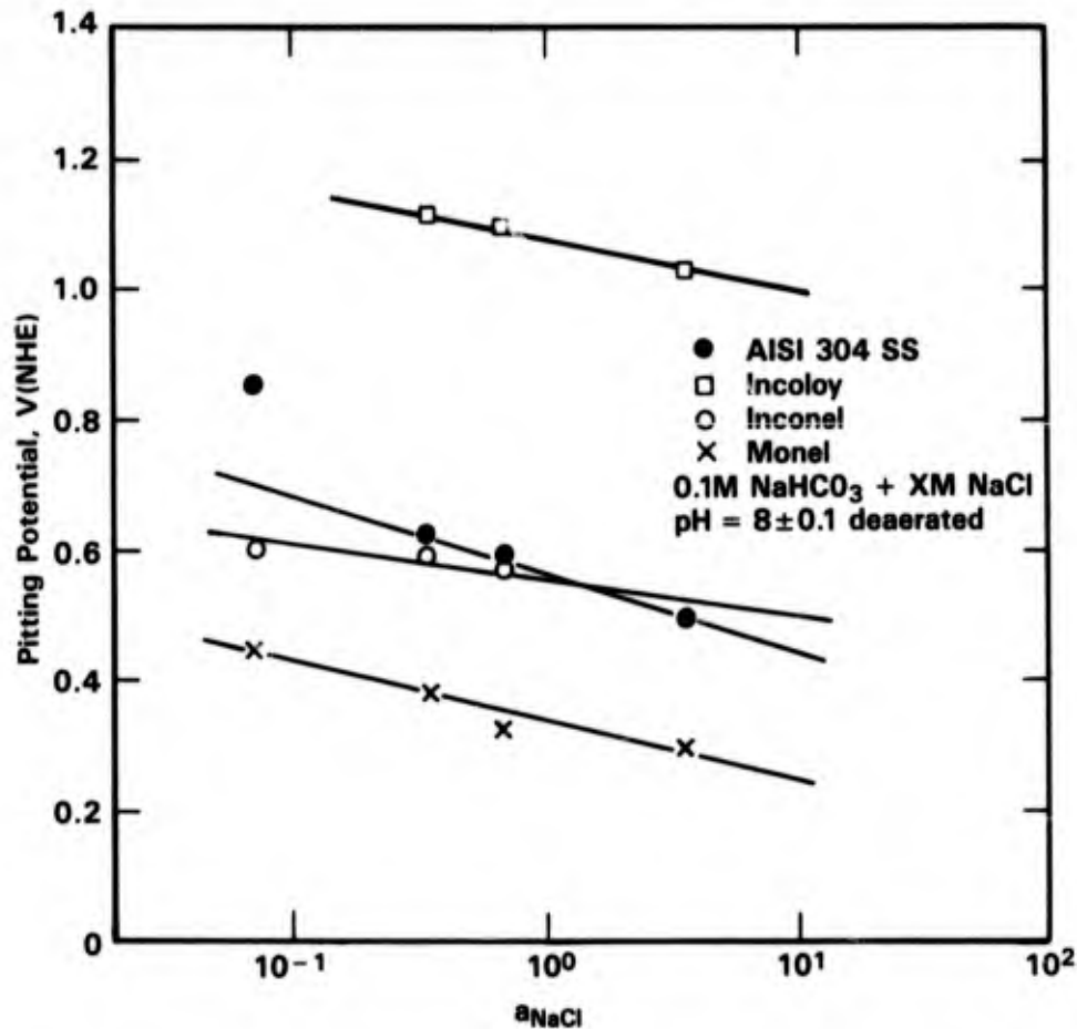
FIGURE 5-12. PITTING POTENTIALS VERSUS \text{NaCl} ACTIVITIES FOR TYPE 304 STAINLESS STEEL, INCOLOY, INCONEL 600, AND MONEL (33)
