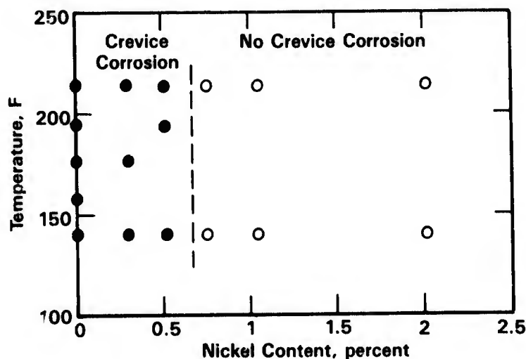
FIGURE 3-1. EFFECT OF THE Ni CONTENT ON THE CREVICE CORROSION RESISTANCE OF TITANIUM IN 6 PERCENT NaCl AQUEOUS SOLUTION AT VARIOUS TEMPERATURES (16)
