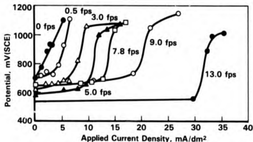
FIGURE 14-1. CATHODIC POLARIZATION OF MILD STEEL IN SEAWATER FLOWING AT DIFFERENT VELOCITIES AT 26 C (6)
