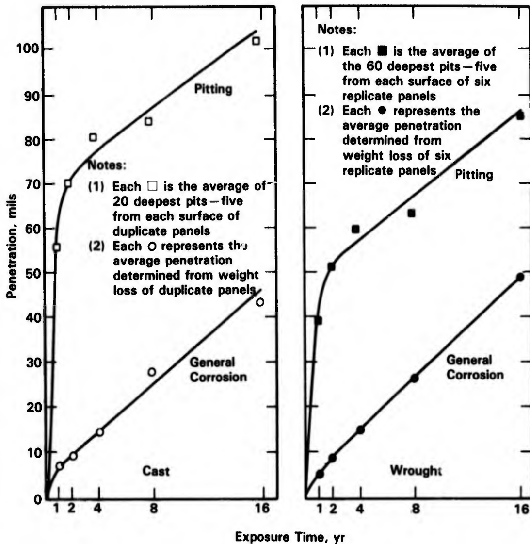
FIGURE 6-15. CURVES SHOWING WEIGHT-LOSS AND PITTING FOR (a) CAST STEEL AND (b) WROUGHT CARBON STEEL CONTINUOUSLY IMMERSSED IN SEAWATER (17)
