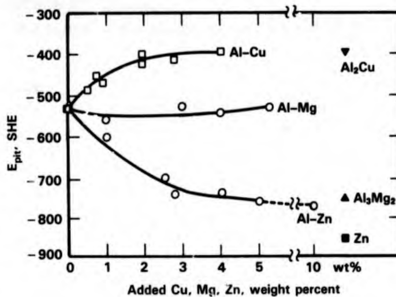
FIGURE 2-18. PITTING POTENTIAL ( E_{pit} ) VALUES AS A FUNCTION OF ALLOY ADDITIONS TO ALUMINUM ALLOYS, COMPARED WITH E_{pit} OF PHASES THAT ARE PRESENT IN ALUMINUM ALLOYS. THE CORROSION MEDIA WAS 1M NaCl FOR Al-Cu, Al-Mg, AND Al-Zn ALLOYS. FOR Al 3 Mg 2 THE E_{pit} CORRESPONDS TO A SOLUTION 0.5M NaCl (59)
