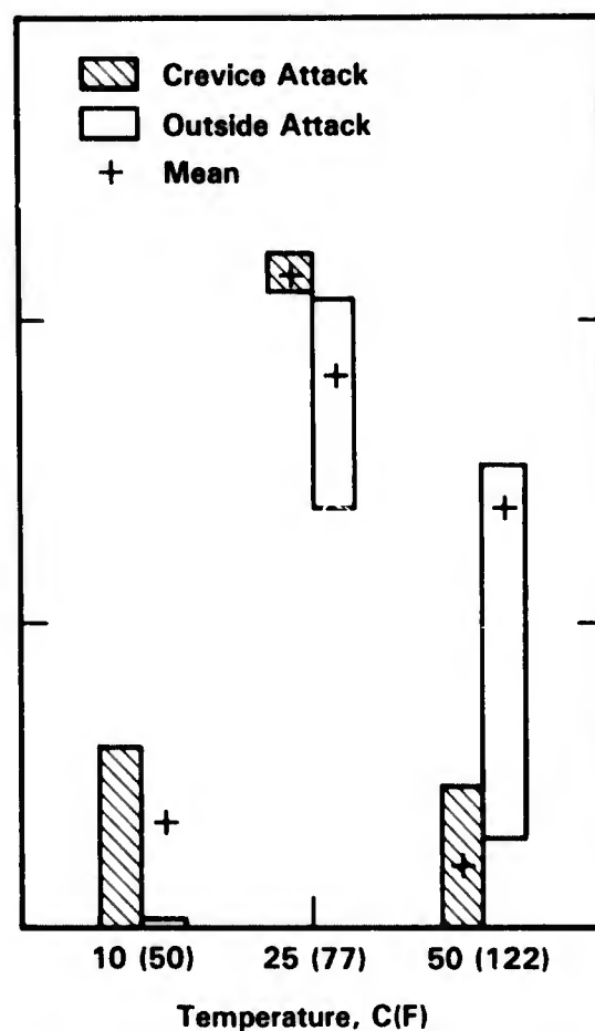
FIGURE 4-7. MAXIMUM DEPTH OF ATTACK FOR 5 SPECIMENS OF TYPE 316 STAINLESS STEEL AFTER 28 DAYS IN SEAWATER (58)
