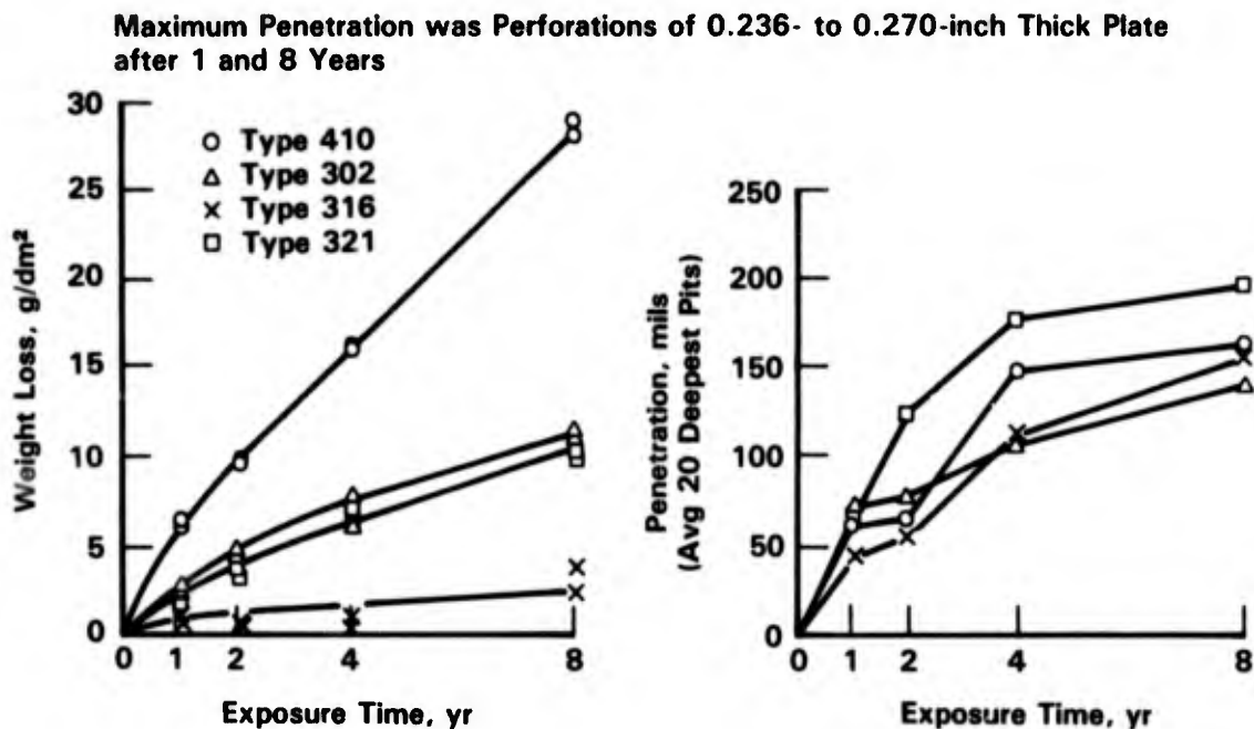
FIGURE 4-3. COMPARATIVE CORROSION OF VARIOUS STAINLESS STEEL ALLOYS CONTINUOUSLY IMMERSSED IN TROPICAL SEAWATER (32)
