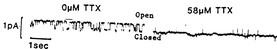
Figure 7: TTX block of BTX-activated Na channel from heart.
