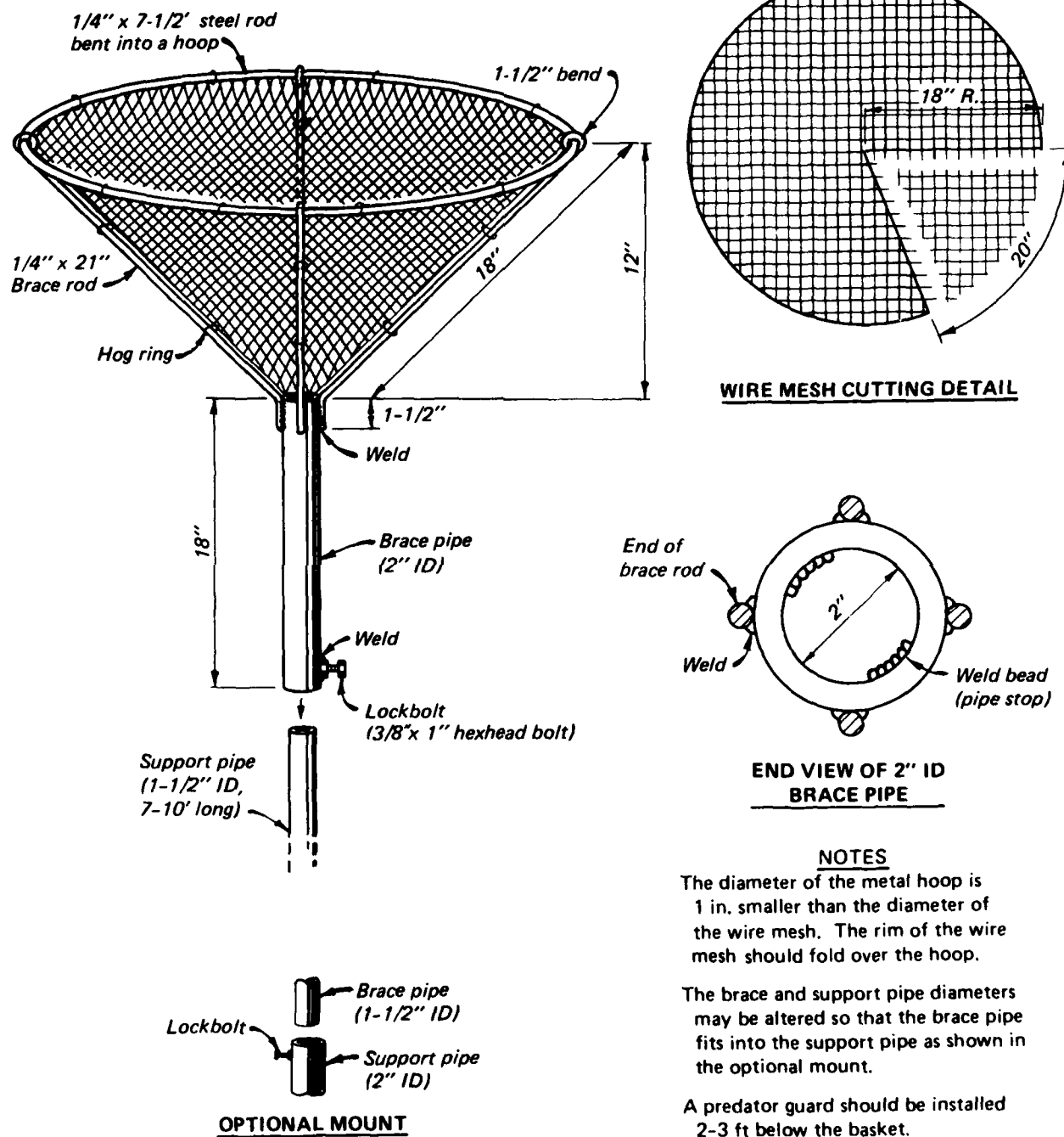
Figure 1. Design specifications for an open basket nest structure for waterfowl (adapted from U.S. Fish and Wildlife Service 1970)
