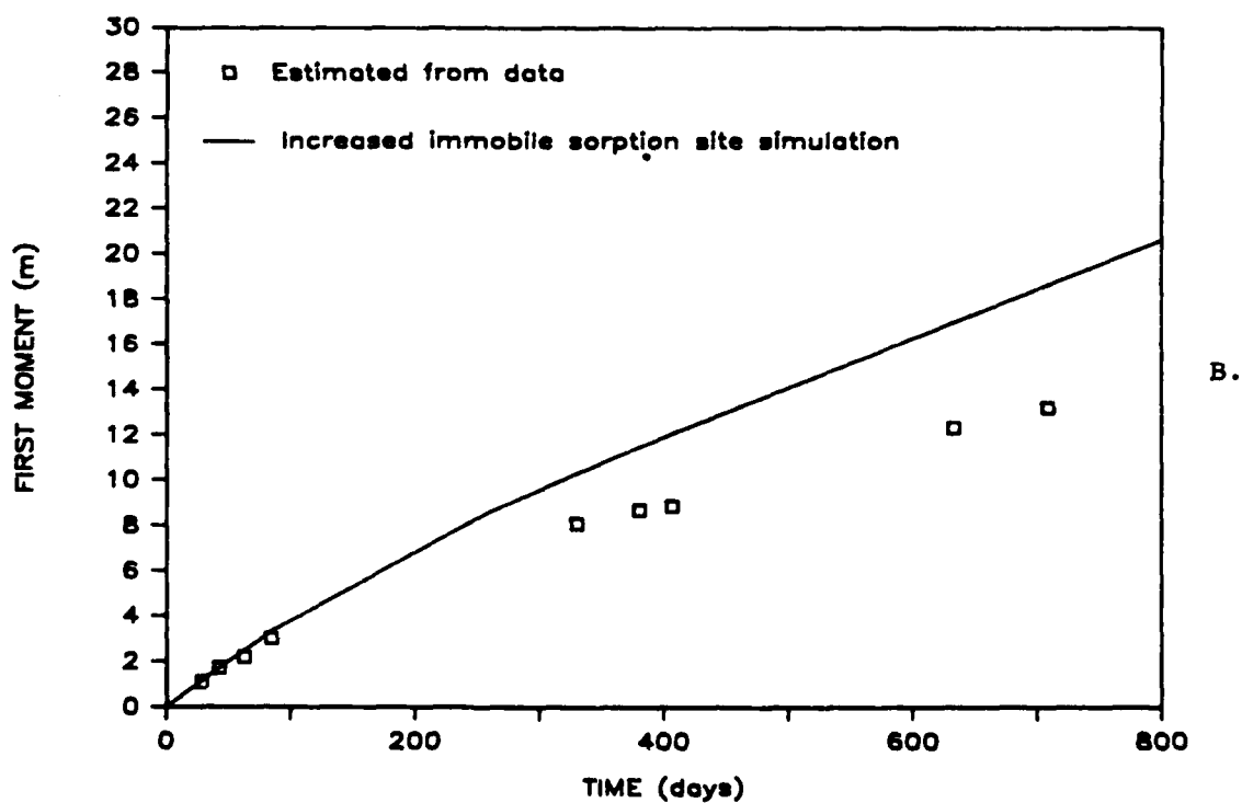
Figure 5.19. Comparison of the tetrachloroethylene mobile region plume: a) Mass in solution, and b) First spatial moment, estimated from synoptic data and simulated using a first-order rate model equivalent to a layered diffusion model, with high sorption capacity within the immobile regions ( f = 0.4 ).
