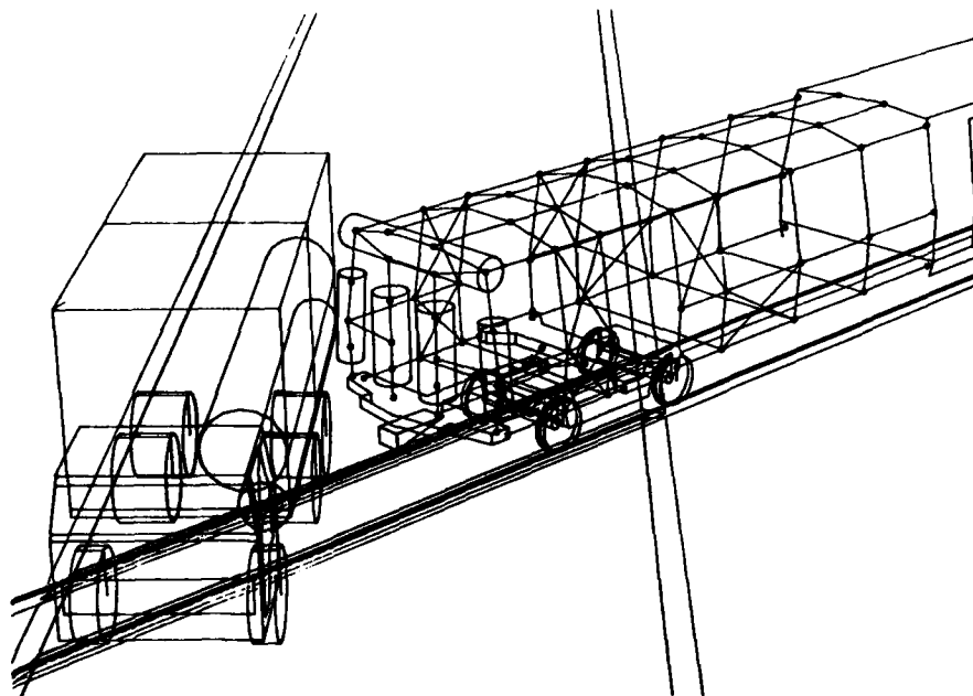
Figure 5. Train to lorry collision model (VEDYAC)
