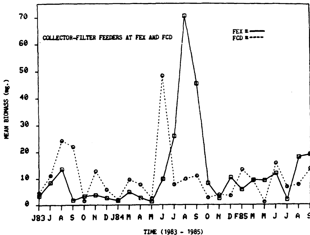
FIGURE 4.12 Changes in predator and filter-feeder biomass (mg./sample) at FEX versus FCD. June, 1983 through Sept., 1985.
