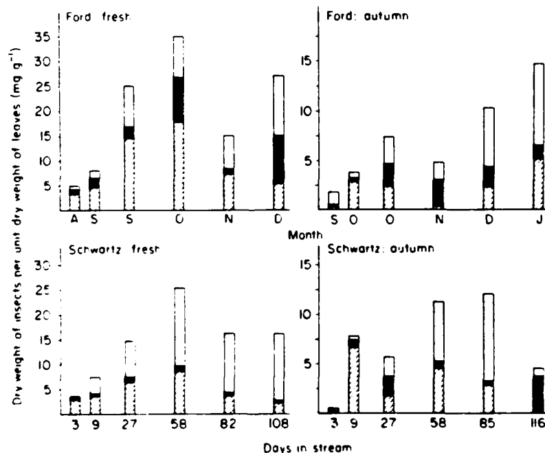
FIG. 4. Mean insect biomass ( \text{mg dry weight} ) per unit leaf biomass ( \text{g dry weight} ) on summer fresh and autumn abscised leaves in the Ford River and Schwartz Creek. Cross-hatched bars: grazer/collectors; black bars: shredders; white, black and cross-hatched bars: all functional feeding groups, including chironomids. Note different y-axes for summer fresh versus autumn abscised leaves.
