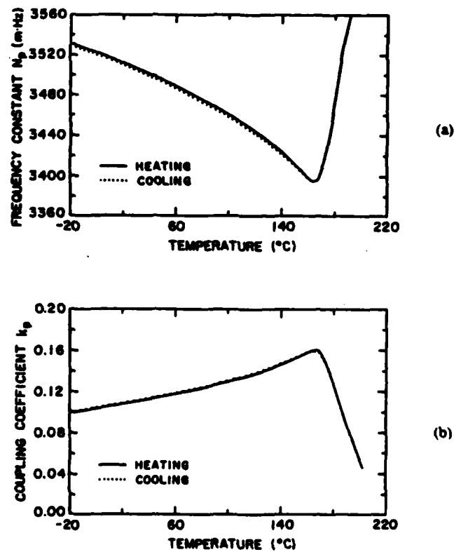
FIGURE 7 Frequency constant N_p , (a) and electromechanical coupling k_p , (b) of \text{Ba}_2\text{TiSi}_2\text{O}_8 single crystal as a function of temperature.
