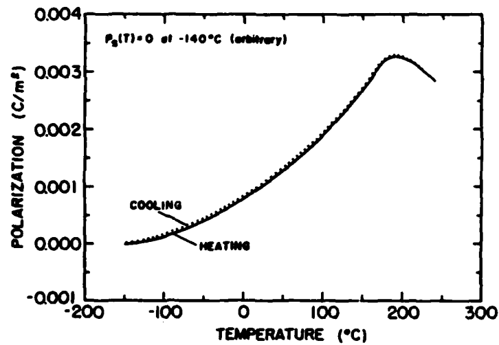
FIGURE 6 Polarization of \text{Ba}_2\text{TiSi}_2\text{O}_8 single crystal as a function of temperature.
