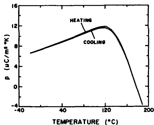
FIGURE 5 Pyroelectric coefficient as a function of temperature for 2BaO-3SiO 2 -TiO 2 glass-ceramics.
