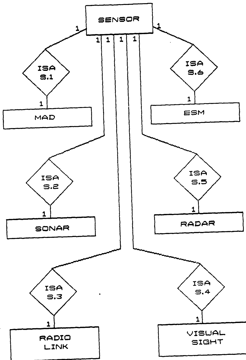
Figure 3.5 ERD for SENSOR
