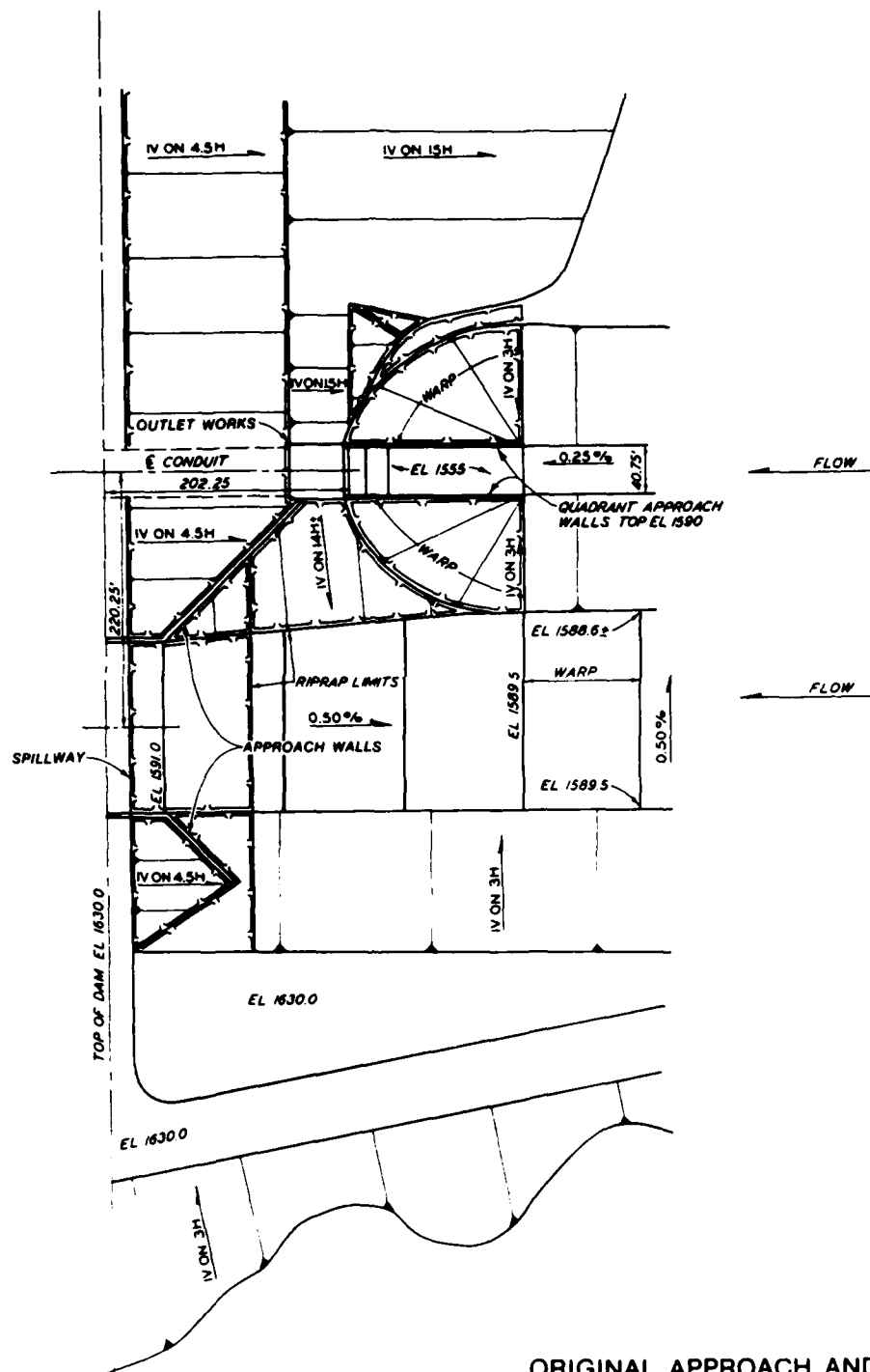
ORIGINAL APPROACH AND PROTECTION DESIGN
