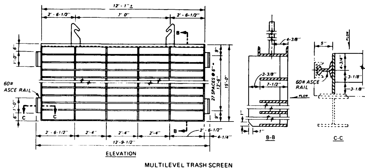
Figure 2. Details of trashrack configuration
