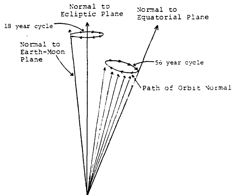
Figure 1D. Path of orbit normal ( J_2 , Sun, Moon)
