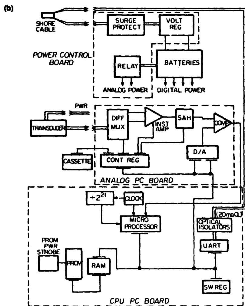
Figure 1 - Wave Measuring System, (a) Pressure Transducer, (b) Block Diagrams of Underwater Data Acquisition System
