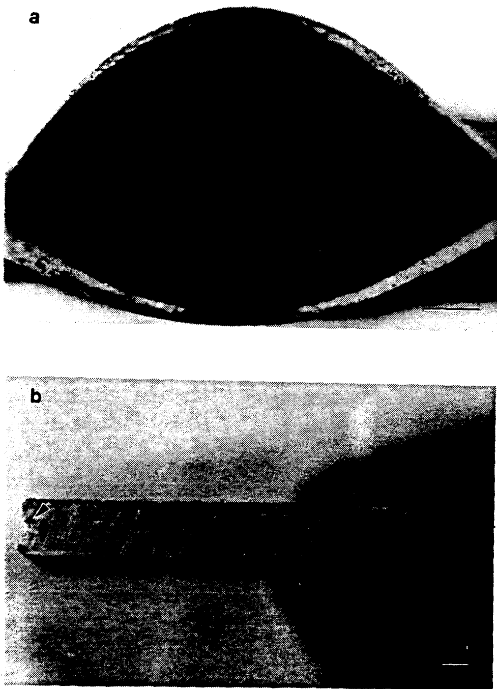
Figure 4.8. Photographs of 300°C warm rolled specimens showing (a) alligatoring due to light reduction during processing and (b) edge of same sample revealing non-uniform working of material.
