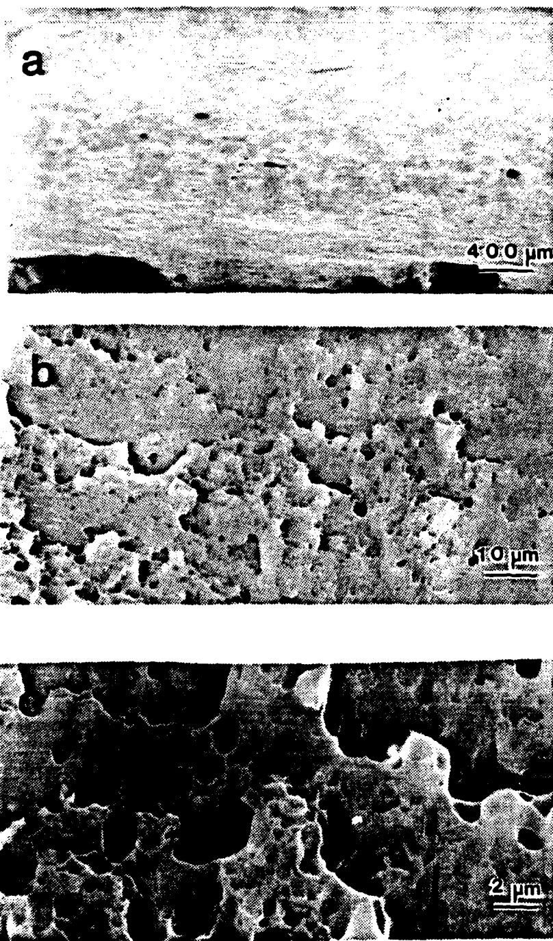
Figure 4.14. SEM micrographs of a test specimen tension tested at ambient temperature following heavy reduction processing. Ductility was 19.0 percent elongation to fracture; fracture surface: (a) 26.5X, (b) 1000X, (c) 4000X.
