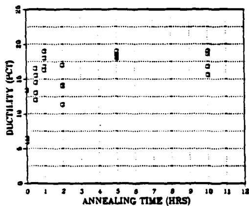
Figure 4.10. Results of ambient temperature tension testing of material processed as in previous work; (a) and (b) are the results of the first series of tests, while (c) and (d) are the second series of tests.
