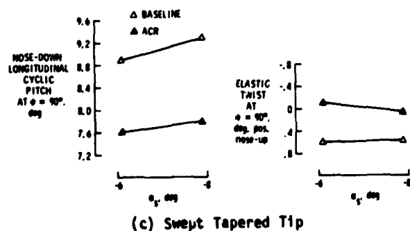
Fig. 11 Advancing blade control angle and elastic twist versus \alpha_s ( \mu = .35 , M_T = .65 , \bar{C}_L/\sigma = .08 ).
