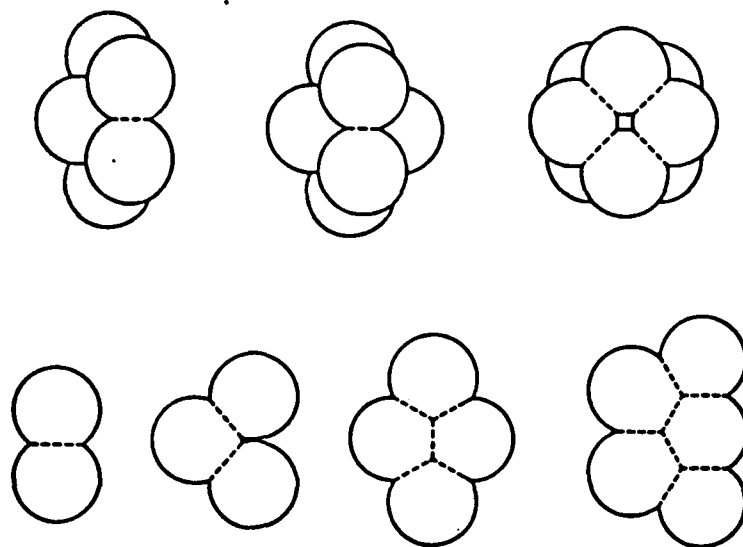
Figure 2. The calculated structures of the pseudopotential clusters for r_c = 4 . The sphere radii describing the atoms are equal to r_c . The cluster with 2 to 5 atoms are planar. In the 6 and 7 atomic clusters the fifth atom of the five-fold ring can not be seen. The 8 atomic cluster consists of the squares of atoms rotated 45 degrees with respect to each other.
