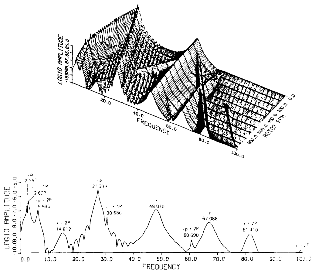
Fig. 10. Response of z_c coordinate to an x initial condition; stiff body, no shaft degree of freedom, 4% mismatched blades. (a) As function of rpm. (b) At 1000 rpm.
