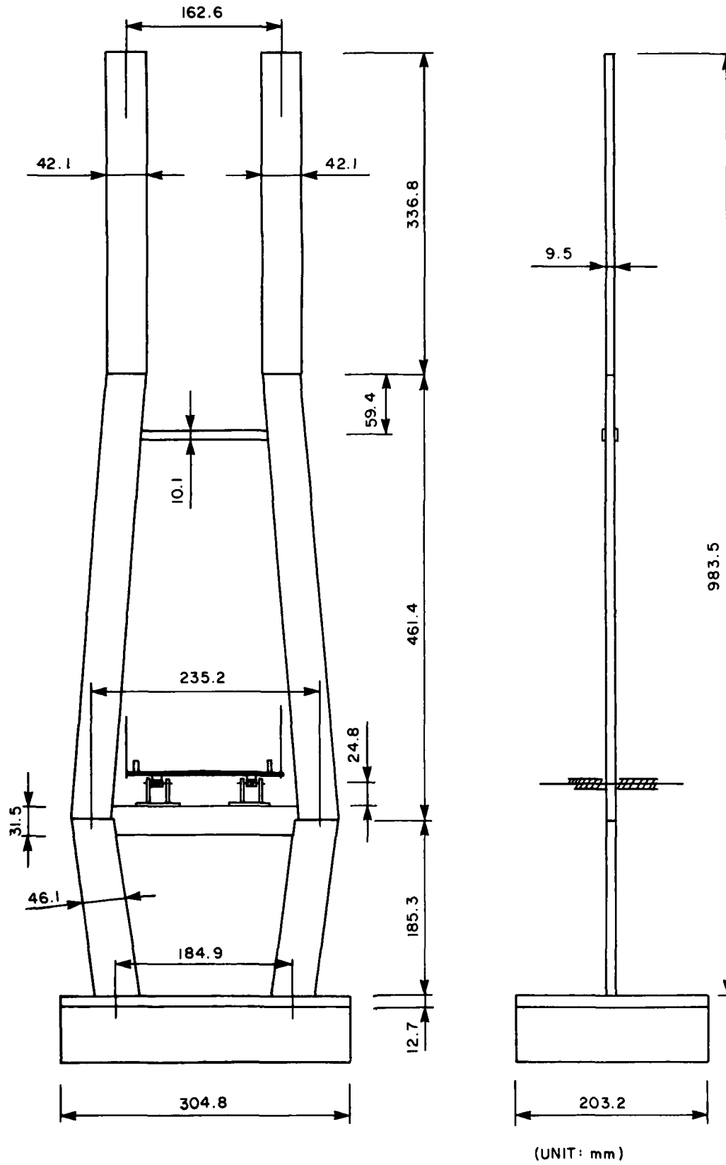
FIG. 4: TOWER (STEEL)
