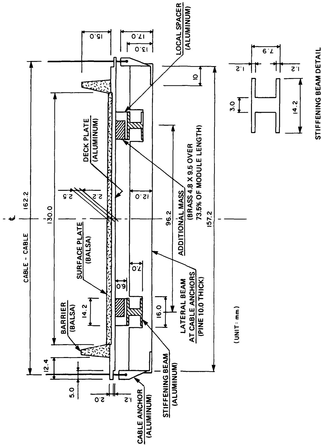
FIG. 5: BRIDGE DECK AND FLOOR SYSTEM WITH CABLES COMMON ELEMENT FOR EACH CONFIGURATION
