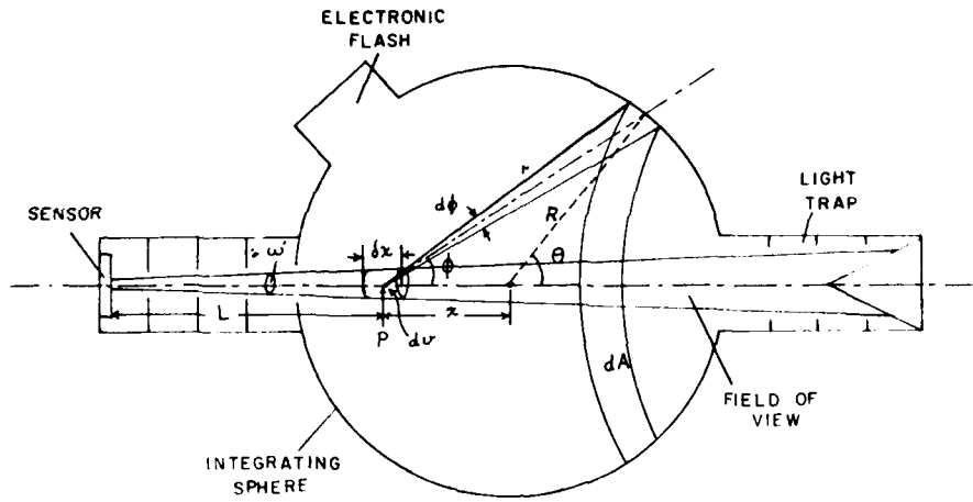
Fig. 7—Schematic of the integrating sphere nephelometer
