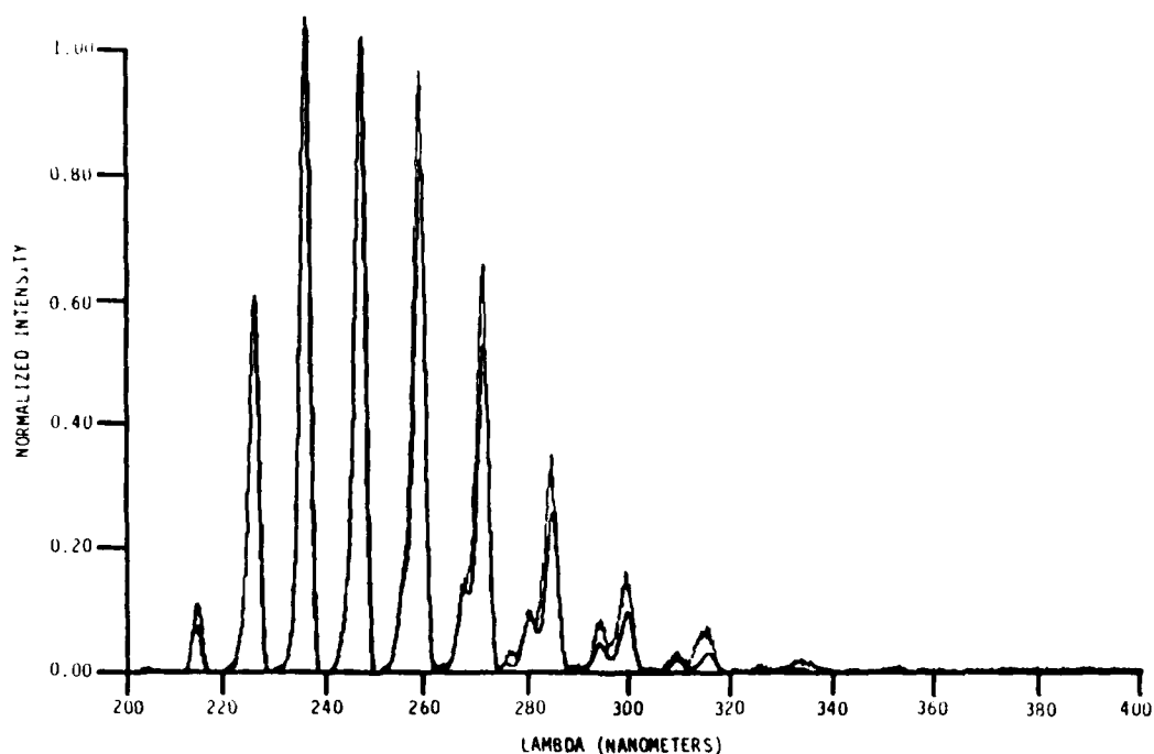
Figure G-4. Experimental (light line) and synthetic (heavy line) spectrum for the NO \gamma -bands assuming a constant electronic transition moment.
