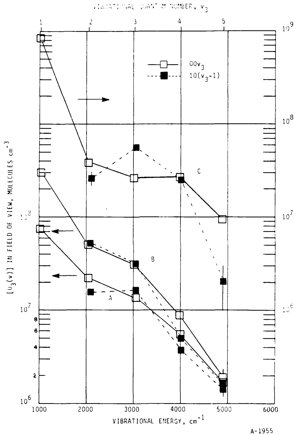
Figure 50. Example \text{O}_3(v) vibrational population distributions, T = 80 \text{ K} . A: 0.24% \text{O}_2 in Ar; b: 1.46% \text{O}_2 in Ar; C: 10.1% \text{O}_2 in Ar.
