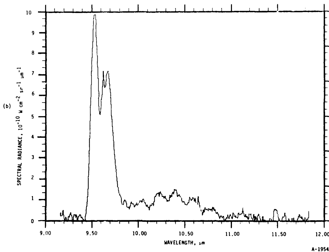
Figure 47. Observed \text{O}_3(\nu) chemiluminescence spectra, medium resolution. T = 80 \text{ K} , spectral resolution = 0.04 \mu\text{m} . (a) 1.0% \text{O}_2 in Ar; (b) 10.0% \text{O}_2 in Ar.
