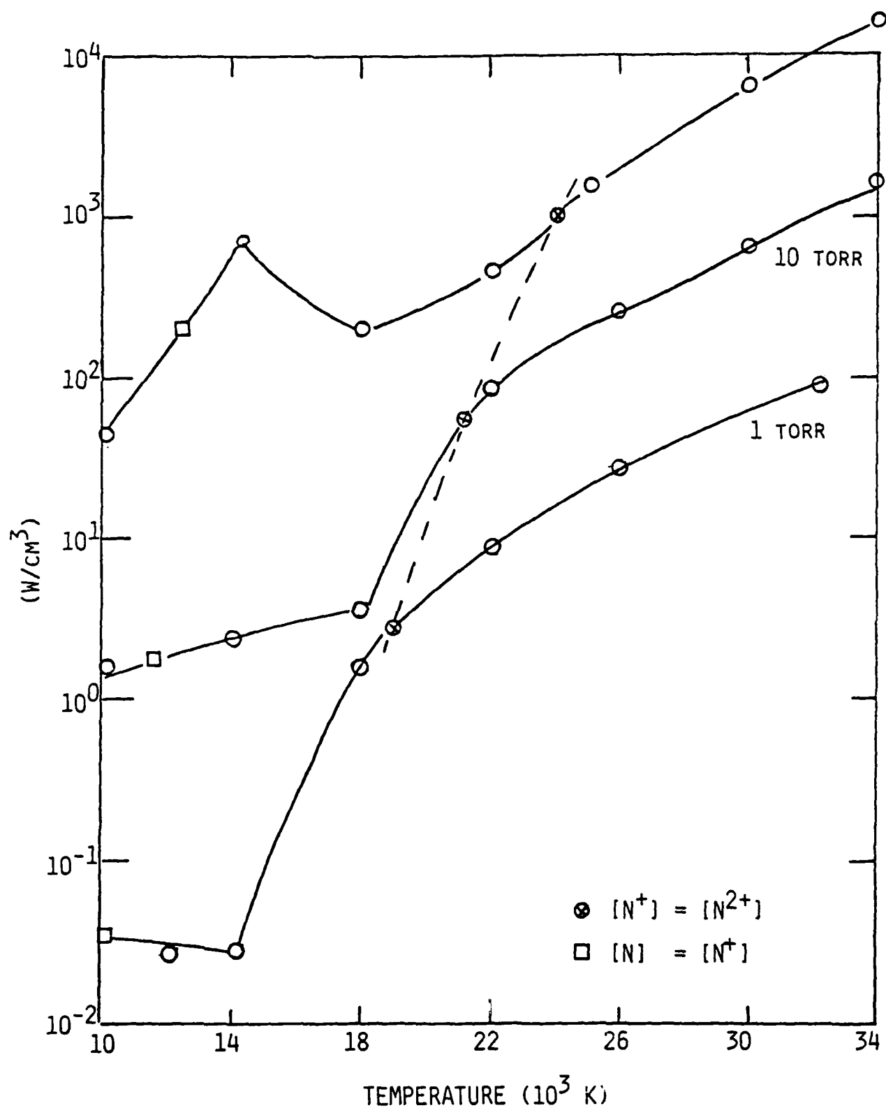
Fig. 32 Integrated emission in the wavenumber band 0 < \bar{\nu} < 250,000 \text{ cm}^{-1} .
