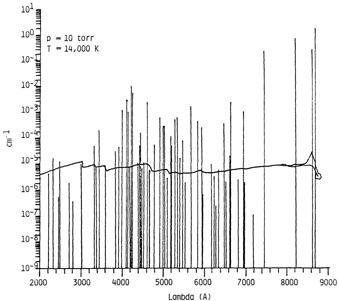
Fig. 30 Absorption coefficient at line center in the 0.2 - 0.9 \mu\text{m} band, nitrogen, T = 14,000 \text{ K} , p = 10 \text{ torr} .
