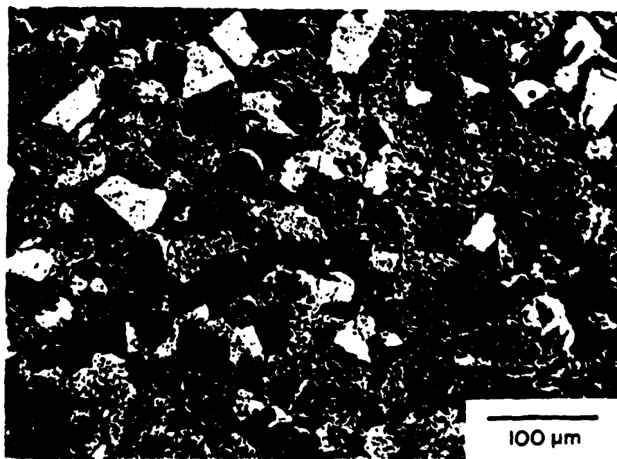
Figure 15. Bimodal Rene 95 powder HIPed at a) 1120°C, 103 MPa, 3 hrs.; b) 1000°C, 10.3 MPa, 3 hrs.
