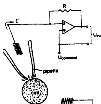
Figure 8. The whole cell configuration of patch clamp pipet with spherical cell.
