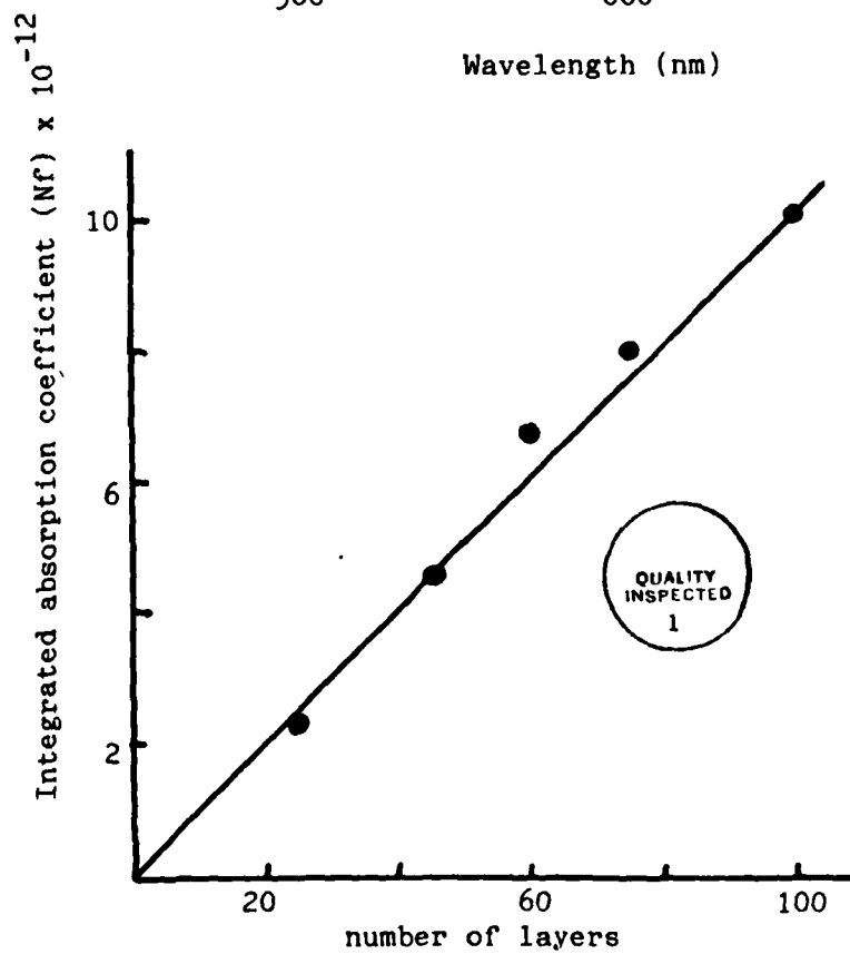
Figure 1 Showing (a) optical absorption coefficient of CuPTC L-B Films on GaP and (b) integrated absorption coefficient (effectively \nu \times oscillator strength f ) under 614 nm band versus number of monolayers.
