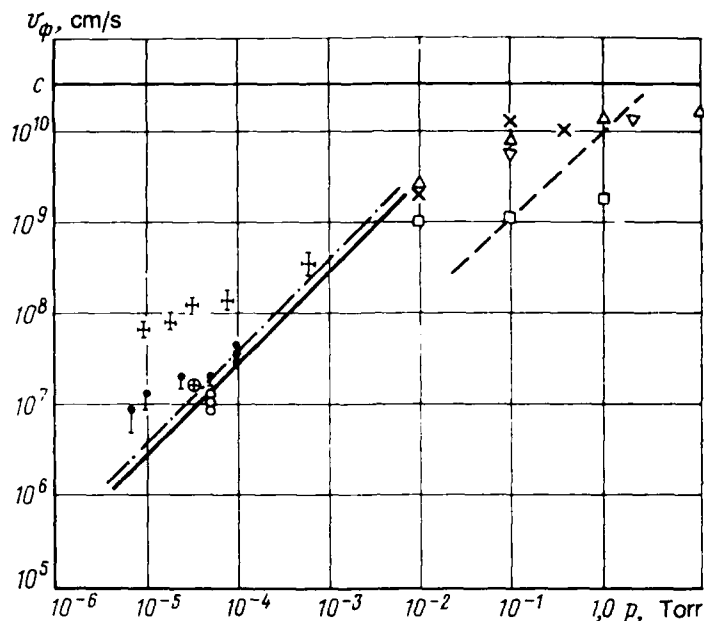
Fig. 12—Velocities of the electron beam propagation as a function of background gas pressure [9]
