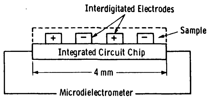
MICRODIELECTROMETRY
