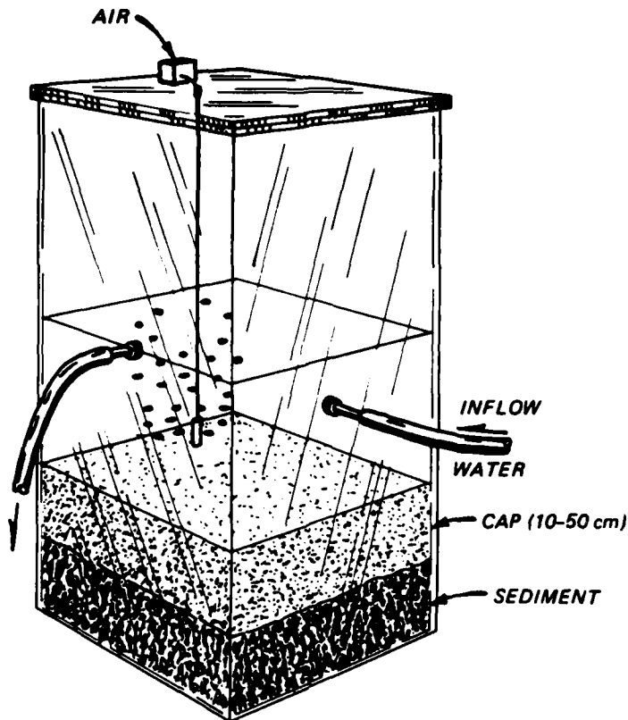
Figure 1. Flow-through reactor units
