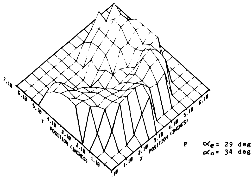
Figure 28. Effect of Alternating Injection Angles on Three-Dimensional Exit Velocity (Continued)
