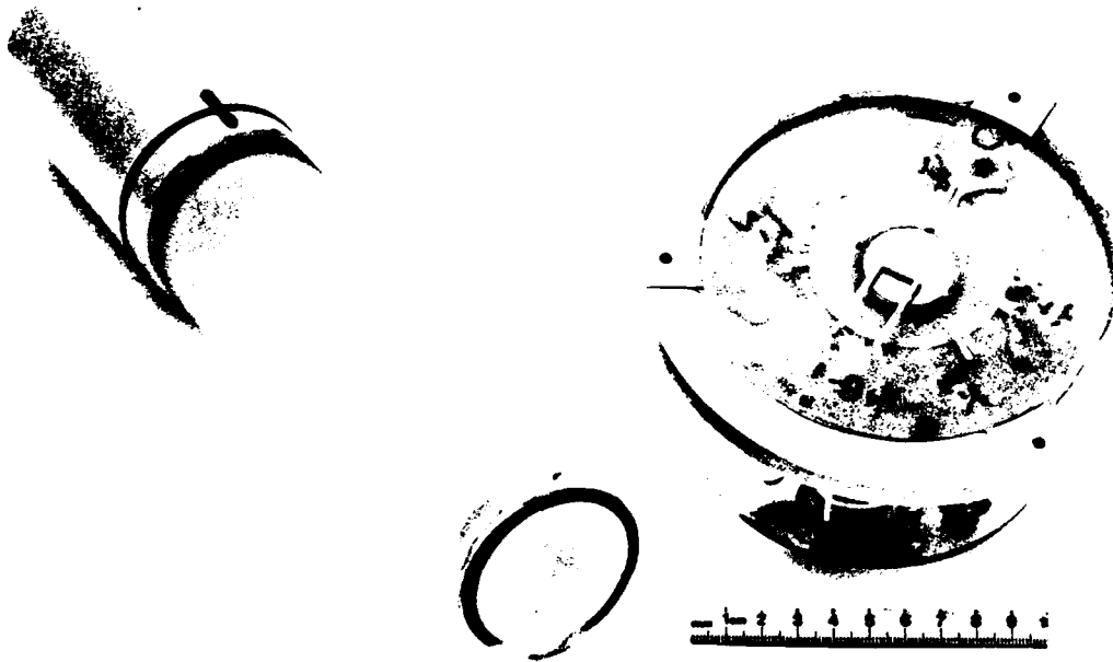
Figure 3. The projectile and target assembly used in the impact experiments. (The vapor-deposited metallic coating on the projectile shorts the vapor-deposited tilt pins on the target to provide a measurement of the impact alignment.)
