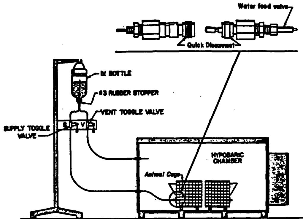
WATER DISPENSING SYSTEM FOR RODENTS IN HYPOBARIC SIMULATOR
