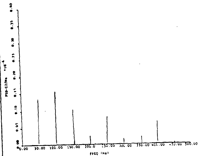
Figure 5. X-Axis Model Vibration
