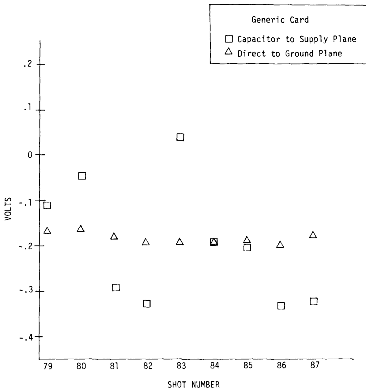
Figure 11b. Measured response of coated generic card
