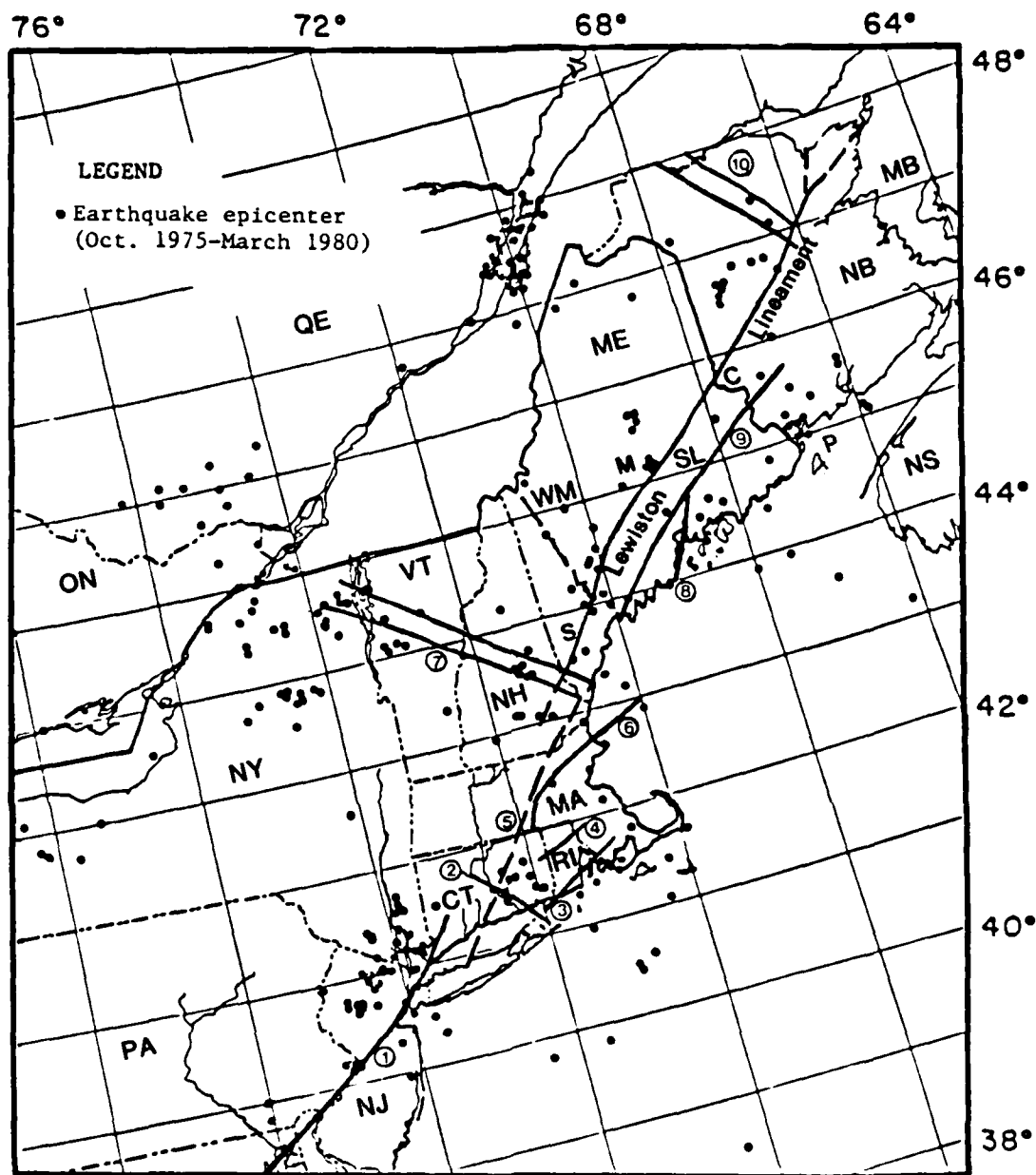
Figure 67. Map of the northeastern U.S. and adjacent Canada showing the Lewiston gravity lineament and other selected interpreted structures found or greatly extended on the basis of magnetic and gravity data. 1. Northern Fall Line; 2. Connecticut River lineament; 3. Watch Hill lineament; 4. North Scituate-Blackstone lineament zone; 5. Higganum dike system; 6. Clinton-Newbury fault zone; 7. Winnepesaukee-Winooski lineament zone; 8. Penobscot lineament; 9. Norumbega fault zone; and 10. Upsalquitch lineament zone. Some geographical locations are: S, Sebago Lake; L, Lewiston; M, Medford; SL, South Lincoln; P, Passamaquoddy Bay; C, Chiputneticook Lakes; MB, Miramichi Bay; WM, West Maine (modified from Barosh, 1982d)
