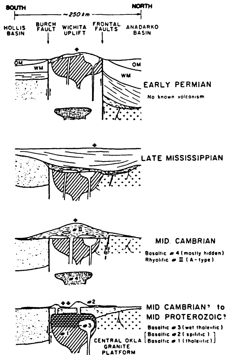
Figure 26. Diagrams showing geologic development of the Wichita Mountains crustal block. View across axis of uplift. Most faults shown at high angle, although the frontal faults are known to dip 30^{\circ} - 40^{\circ} to south (see Brewer, this guidebook). Strike-slip movement not precluded. Rhyolitic I = shallow older basement granites, perhaps equivalent to eastern Arbuckle province. Basaltic 1 = Glen Mountains Layered Complex. Basaltic 2 = Navajoe Mountain Basalt-Spilitic Group. Basaltic 3 = Roosevelt Gabbros. Rhyolitic II = Carlton Rhyolite Group and Wichita Granite Group. Basaltic 4 = late diabase. Short, heavy arrows indicate net motion of land surface, by subsidence, uplift, or erosion. (Gilbert, 1982, Fig. 5)
