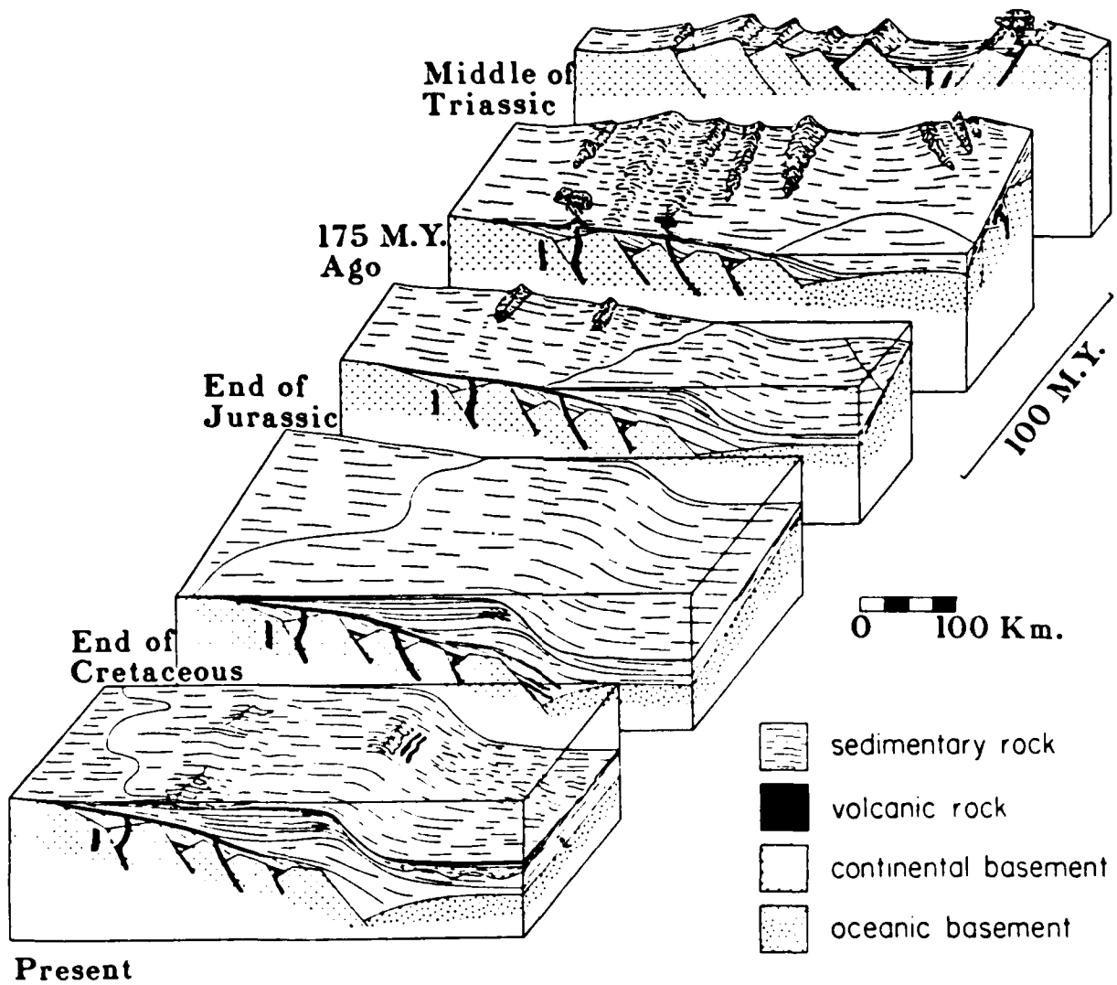
Figure 11. Block diagrams showing historic development of the continental margin near Charleston, South Carolina (Dillon and others, 1979, Fig. 13)
