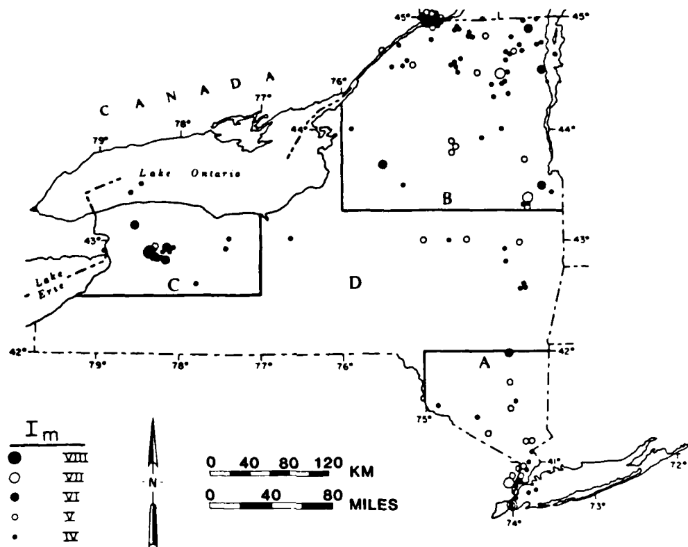
Figure 98. Epicentral map of New York showing areas of relatively greater seismicity: A. Hudson Highlands-Raritan Bay; B. Adirondack Mountains; and C. Attica
