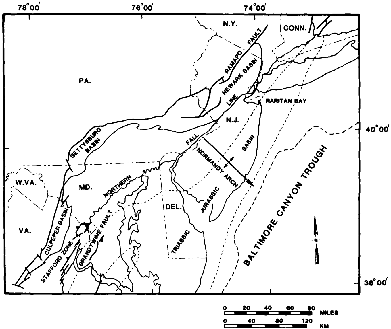
Figure 52. Map of Raritan Embayment and surrounding region showing location of early Mesozoic basins, oceanic fracture zones and selected geologic features (Wentworth and Mergner-Kefer, 1983)
