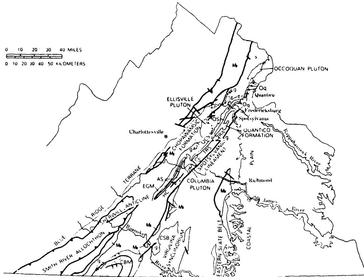
Figure 51. Map of Virginia showing early Mesozoic basins and selected geologic features (Pavlidis, 1981, Fig. 1)
