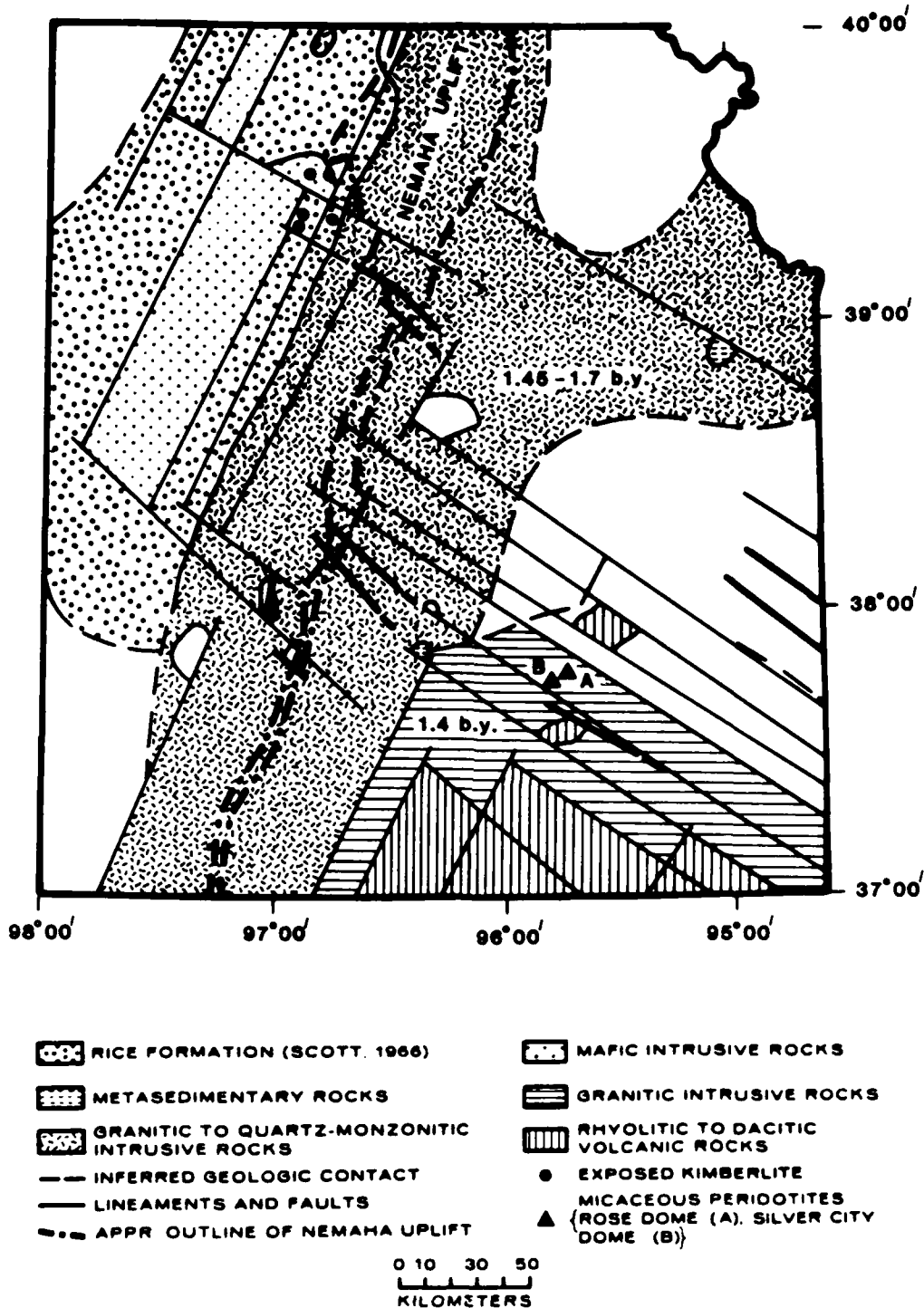
Figure 28. Map of eastern Kansas showing geologic interpretation of the Precambrian basement rocks. Blank spaces represent areas for which no information regarding basement rock types is available (Berendsen and others, 1981, Fig. 9)
