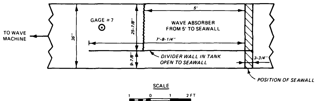
Figure 4. Plan view of Configuration 1, seawall with no fronting revetment
