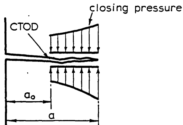
(b) Crack with closing pressure
