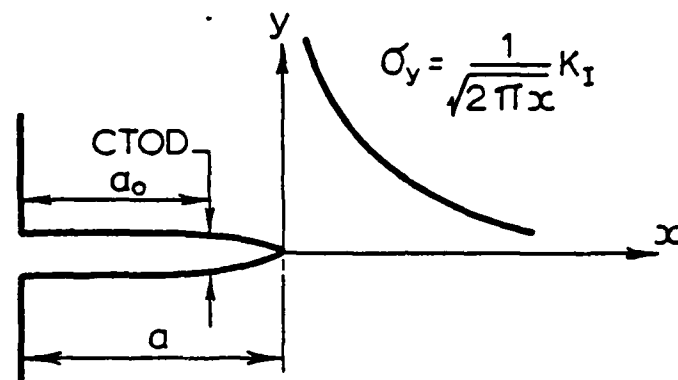
(a) Effective Griffith crack
