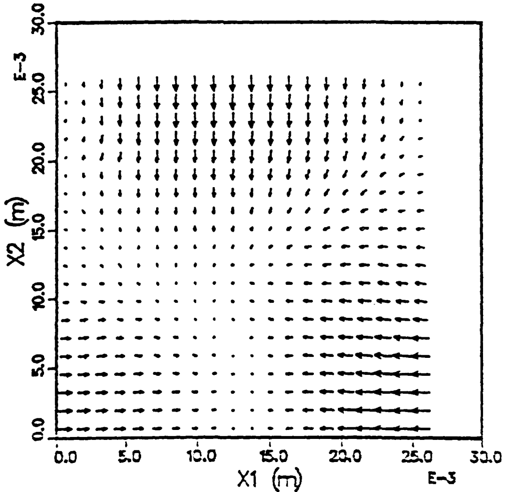
Figure 11. Transverse Electric Fields in Cavity of Antisymmetric CCTWT
