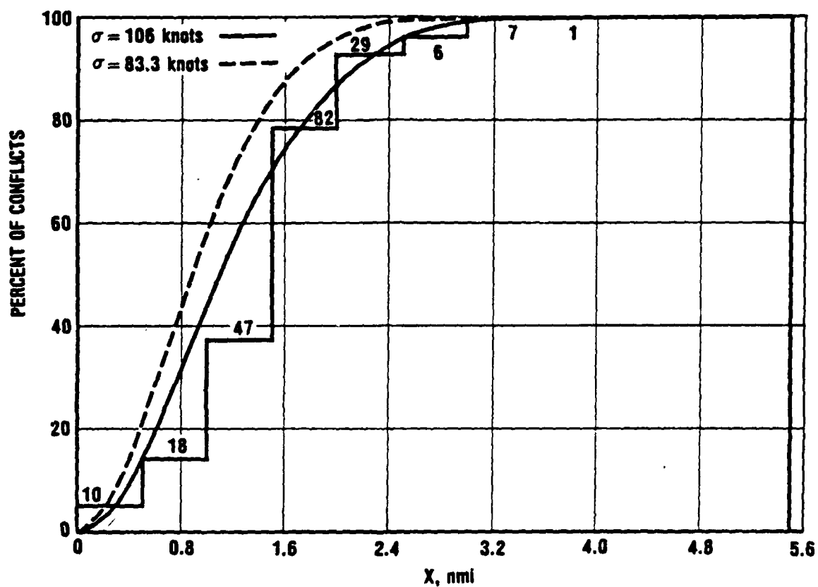
FIGURE A-3. Percent of conflicts with separation at beginning of conflict less than X.
