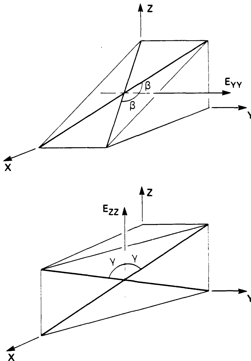
Fig. 9. The use of beta and gamma for determining E_{yy} and E_{zz} .
