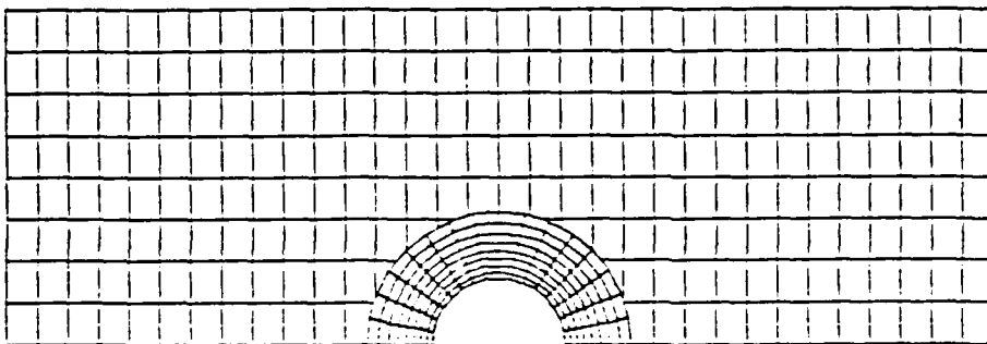
Figure 3-3 Patched Grid
