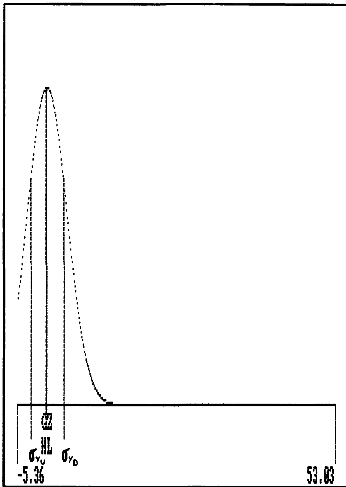
Figure 14. Plot of Crosswind Distribution: t_a=3hr
