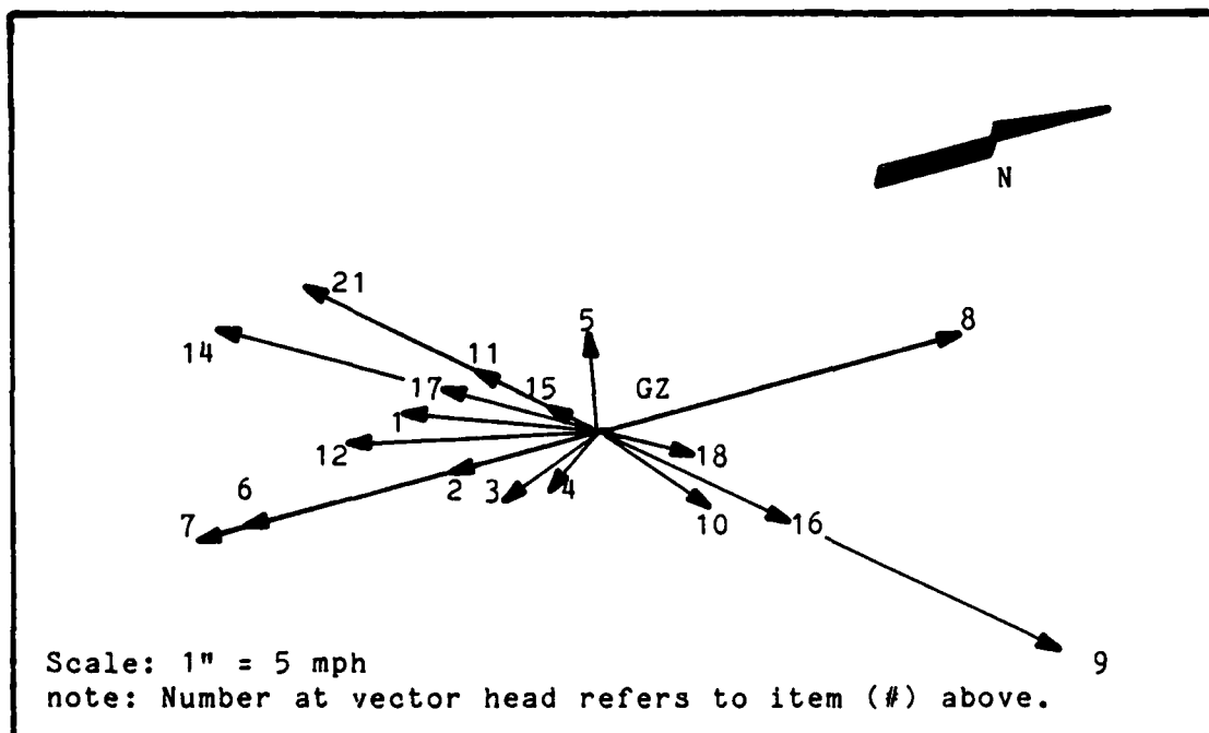
Figure 7. Observed Nevada Shear above Ground Zero
