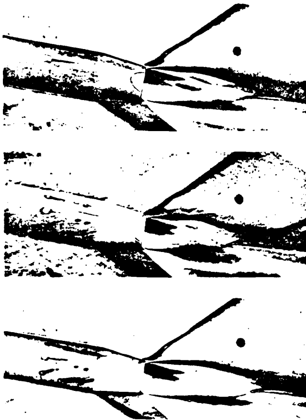
Fig. 22 Oil Flow and Schlieren Photographs at \alpha = -10^\circ and P_{01}/P = 1.00 MPa for Freon (Prototype) and Air (Model) Nozzles
