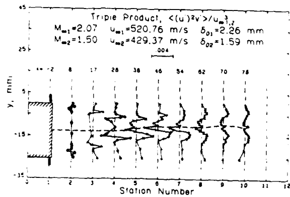
Figure 10. Turbulent triple product
