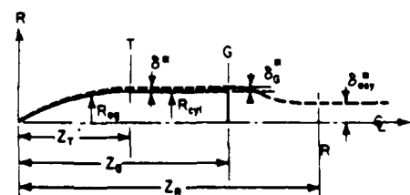
Fig. 2 Equivalent body configuration.
