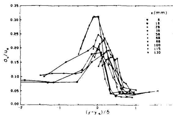
Fig. 8 Streamwise turbulent intensity distributions.
