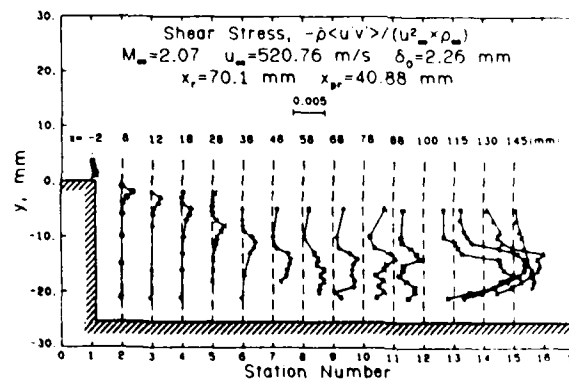
Fig. 9 Turbulent shear stress profiles.
