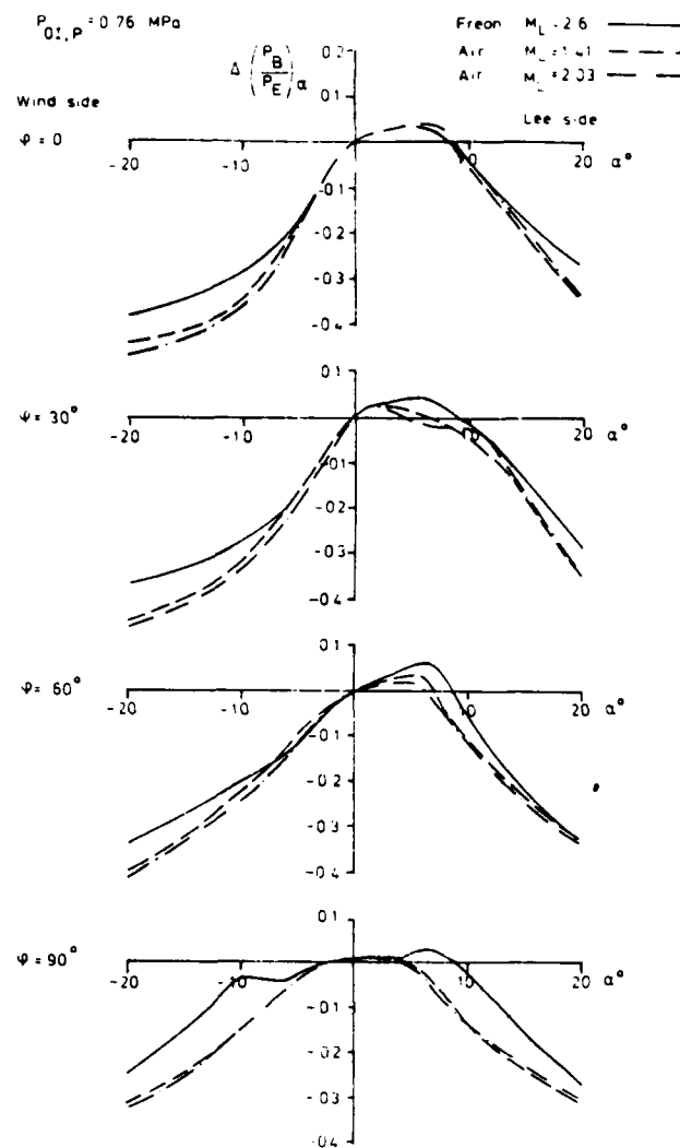
Fig. 17 Effect on Base Pressure Ratio of Angle of Attack \Delta(P_B/P_E)_\alpha = (P_B/P_E)_\alpha - (P_B/P_E)_\alpha=0 versus Angle of Attack \alpha at Stagnation Pressure P_{01,P} = 0.76 MPa
