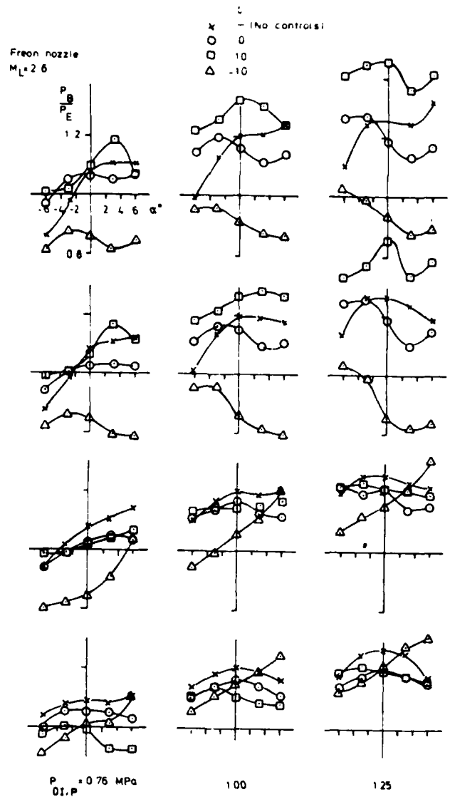
Fig. 23 Base Pressure Ratio for Freon (Prototype) M_L = 2.6 Nozzle versus Angle of Attack \alpha for Different Control Angles \delta , Jet Stagnation Pressures P_{01} and Circumferential Angles \phi
