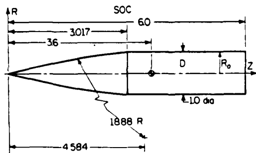
Fig. 1 A six-caliber secant-nose-cylinder projectile.
