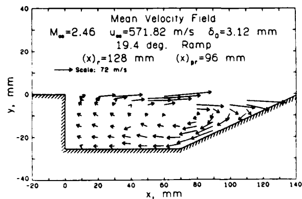
Fig. 7 The recirculating flow mean velocity vector field.
