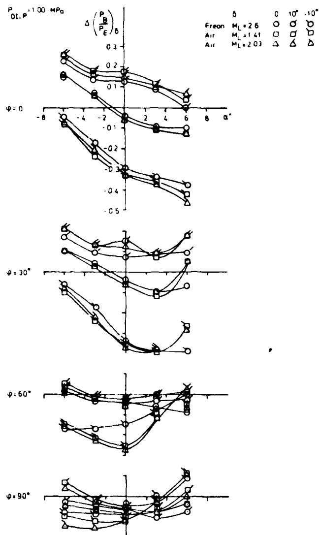
Fig. 27 Effect on Base Pressure Ratio of Controls \Delta(P_B/P_E)_{\delta} = (P_B/P_E)_{\text{with controls}} - (P_B/P_E)_{\text{without controls}} versus Angle of Attack \alpha at Stagnation Pressure P_{01,P} = 1.00 \text{ MPa}
