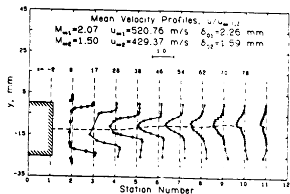
Figure 3. Streamwise mean velocity profiles ( u_{u1,2} means u_{u1} for the upper flow and u_{u2} for the lower flow)
