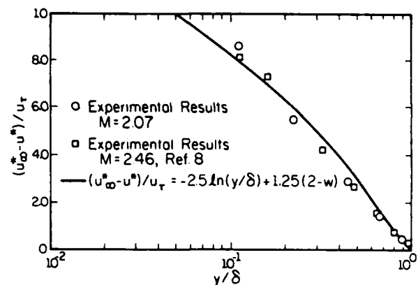
Fig. 2 Boundary layer mean velocity profile and generalized curve of Maise and McDonald [17].
