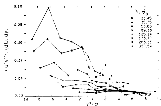
Fig. 15 Kinematic eddy viscosity values for the ramp configuration.
