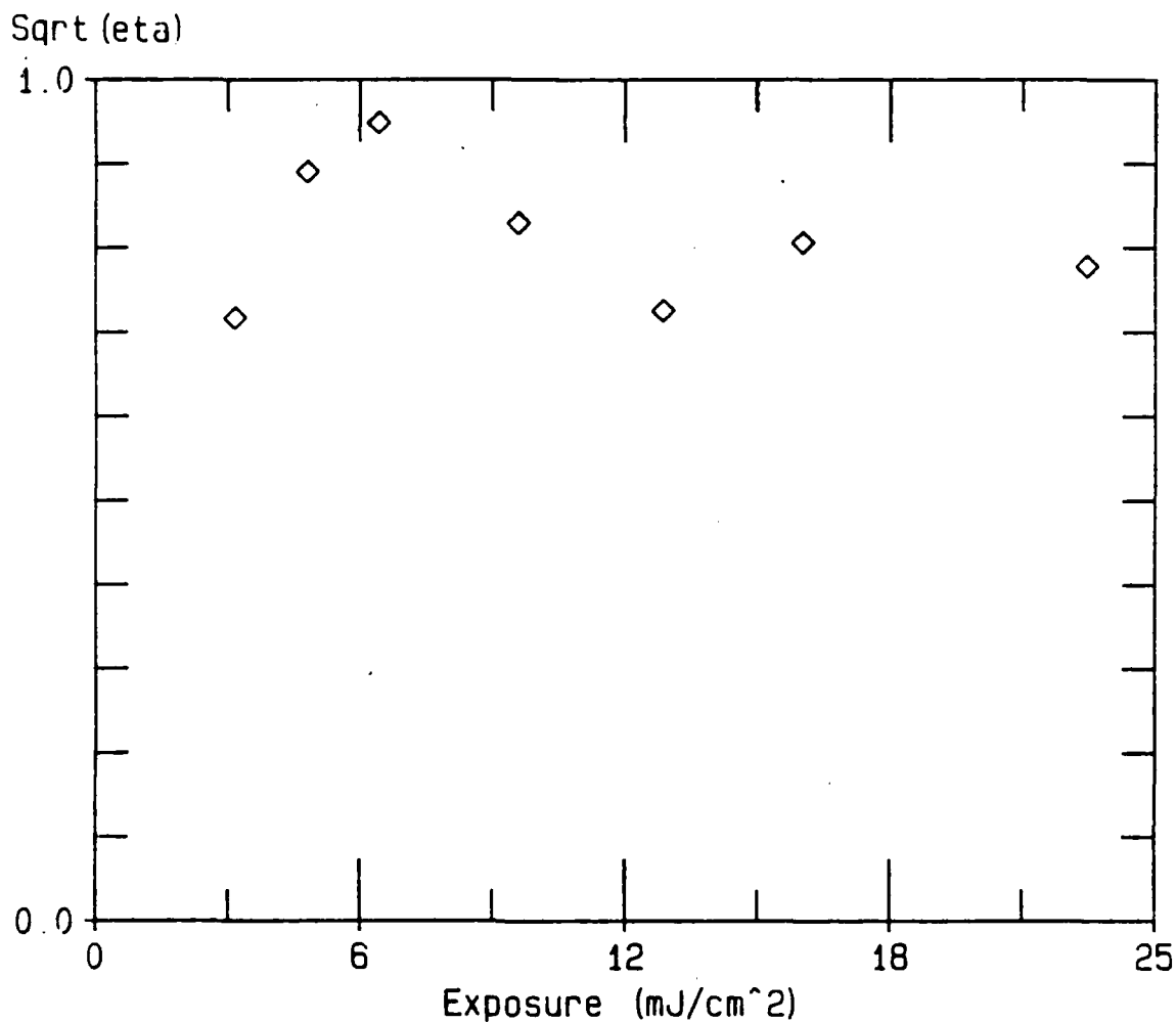
Figure 3-4. \sqrt{\eta} vs. E_0 for \theta_R = \theta_O = 16 . V = 1.0 .
